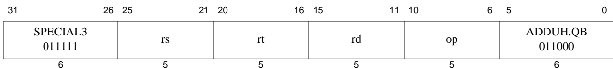
Figure 5.11 SPECIAL3 Encoding of ADDUH.QB Instruction Sub-classes
