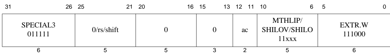
Figure 5.10 SPECIAL3 Encoding Example for EXTR.W Instruction Sub-class Type 3
