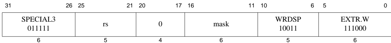
Figure 5.9 SPECIAL3 Encoding Example for EXTR.W Instruction Sub-class Type 2
