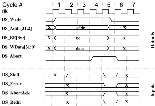
Figure 25 Aborted Write (Multi Cycle)
