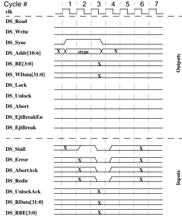
Figure 19 Sync (One Waitstate)
