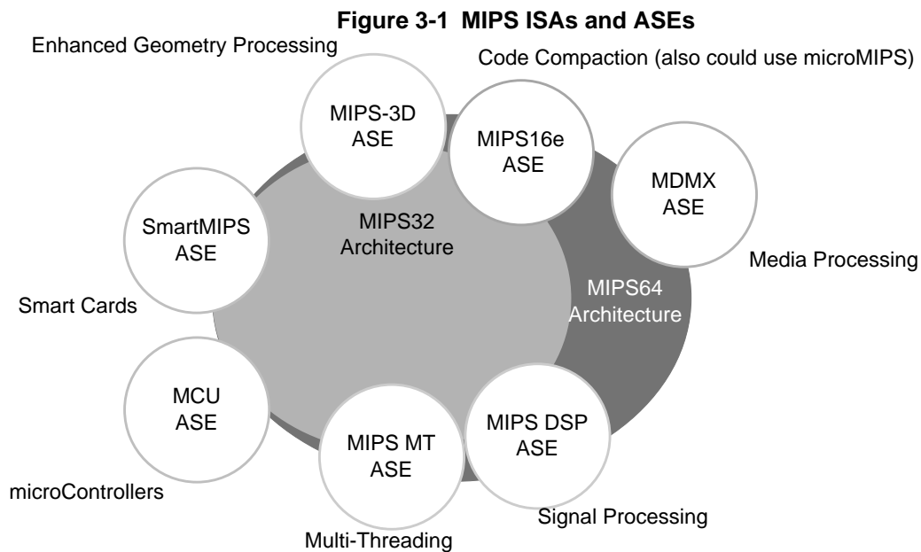
Figure 3-1 shows how ASEs interrelate with the MIPS32 and MIPS64 ISAs.
