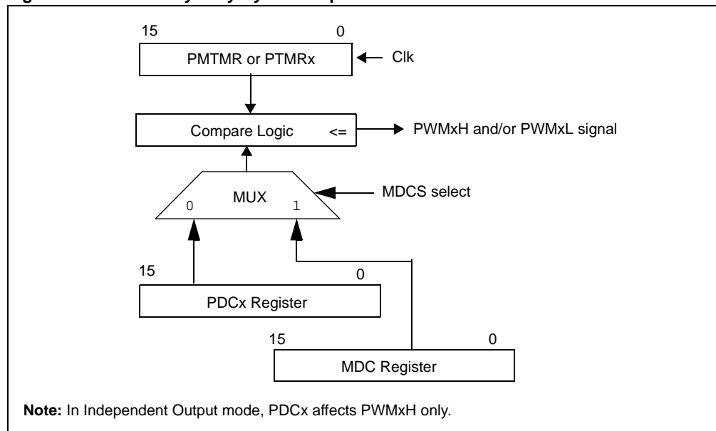
Figure 43-12: Primary Duty Cycle Comparison
