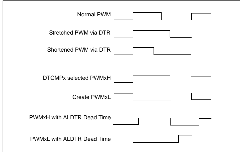
Figure 43-40: Dead-Time Compensation
