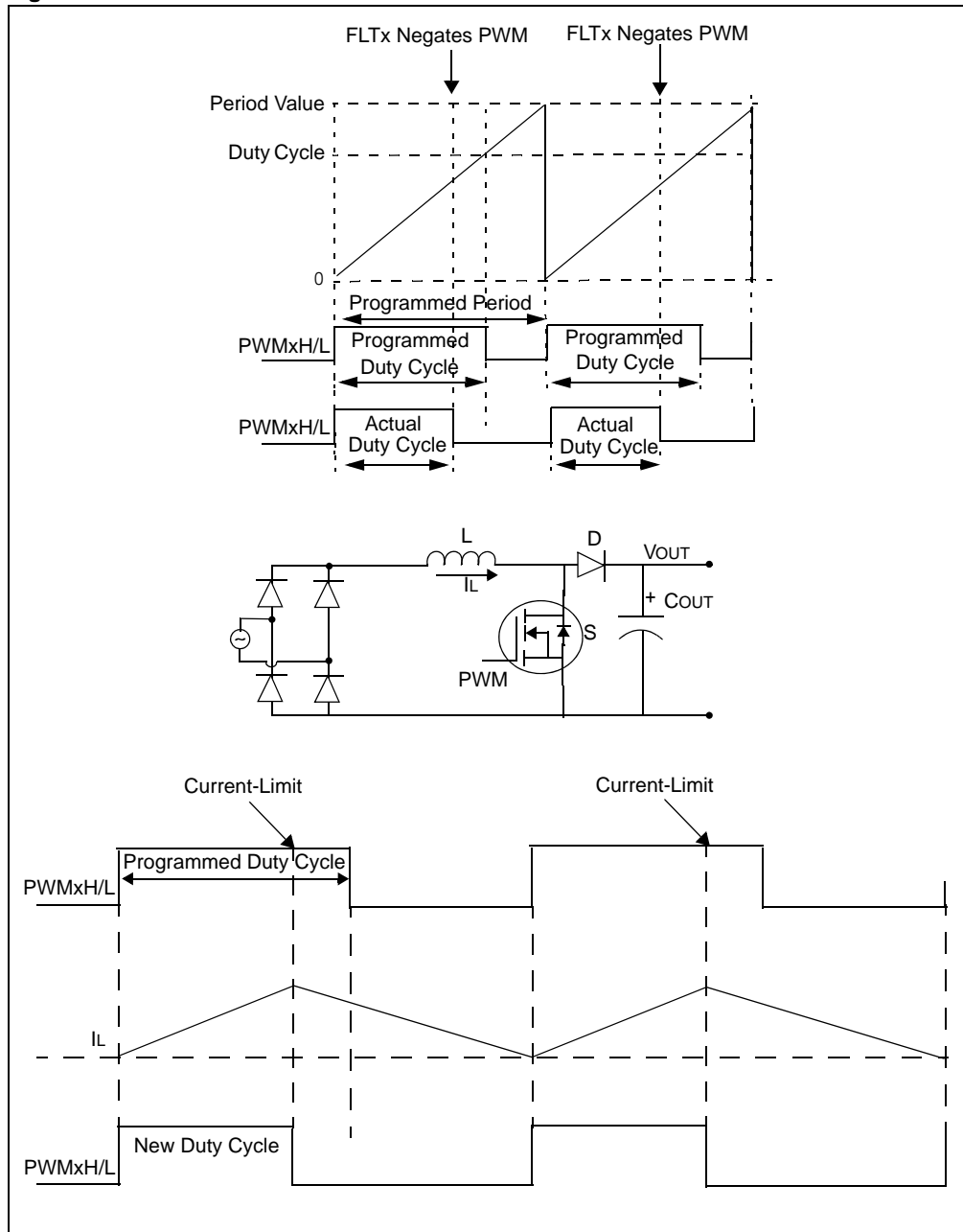
Figure 43-54: Current-Limit PWM
