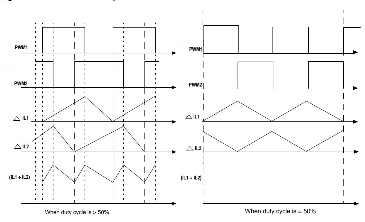
Figure 43-50: Interleaved PFC Operational Waveforms
