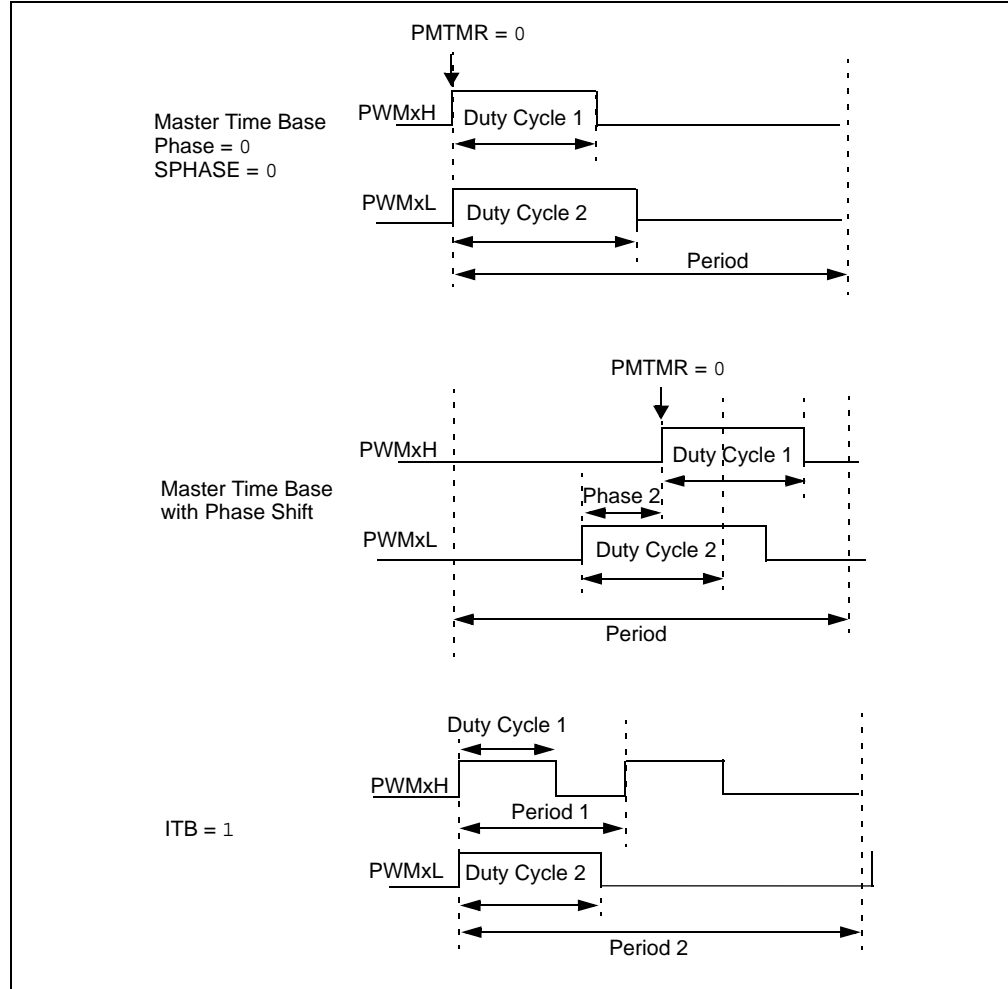
Figure 43-32: True Independent PWM Output Mode
