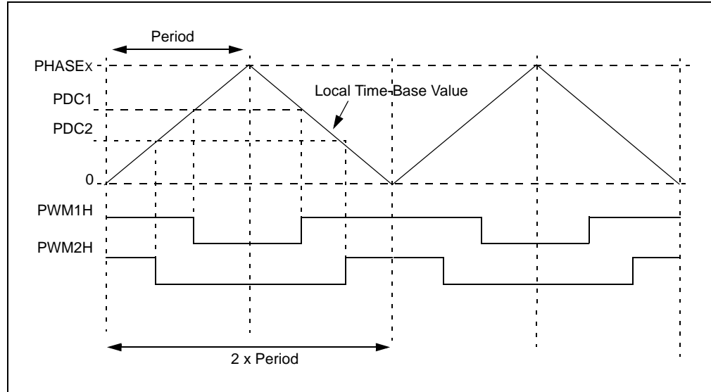
Figure 43-6: Center-Aligned PWM Mode
