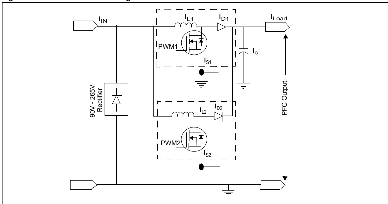
Figure 43-49: Interleaved PFC Diagram
