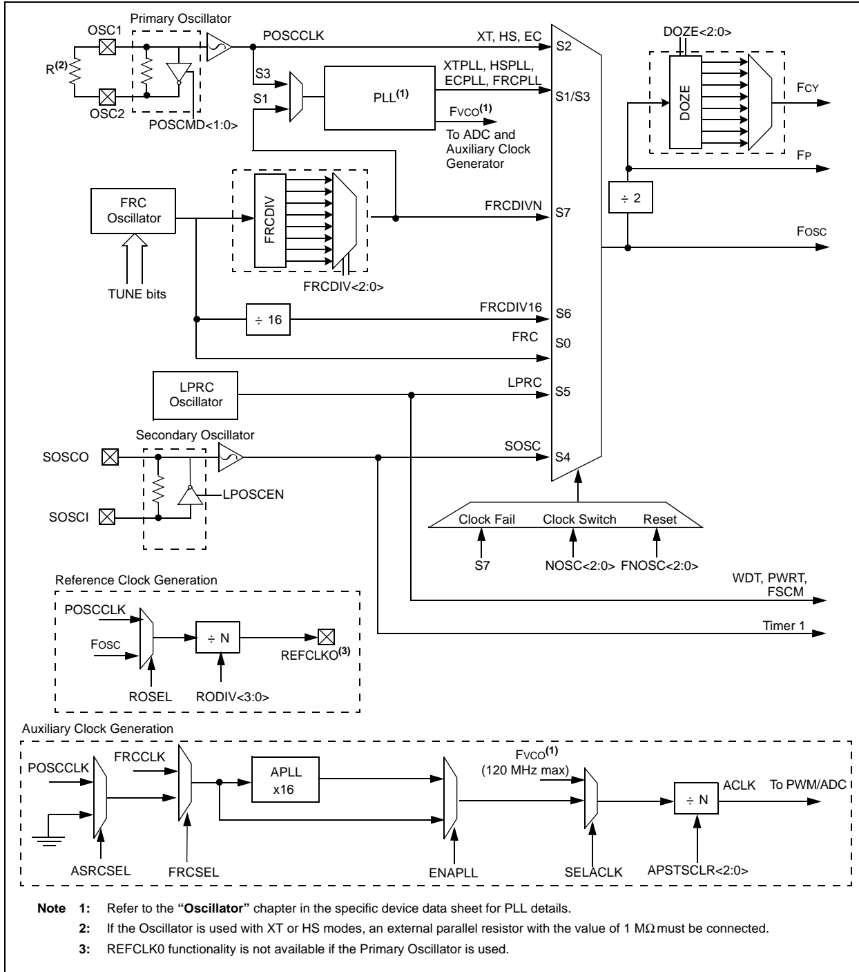
Figure 43-3: Oscillator System
