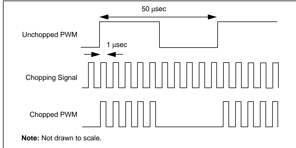
Figure 43-41: High-Frequency PWM Chopping
