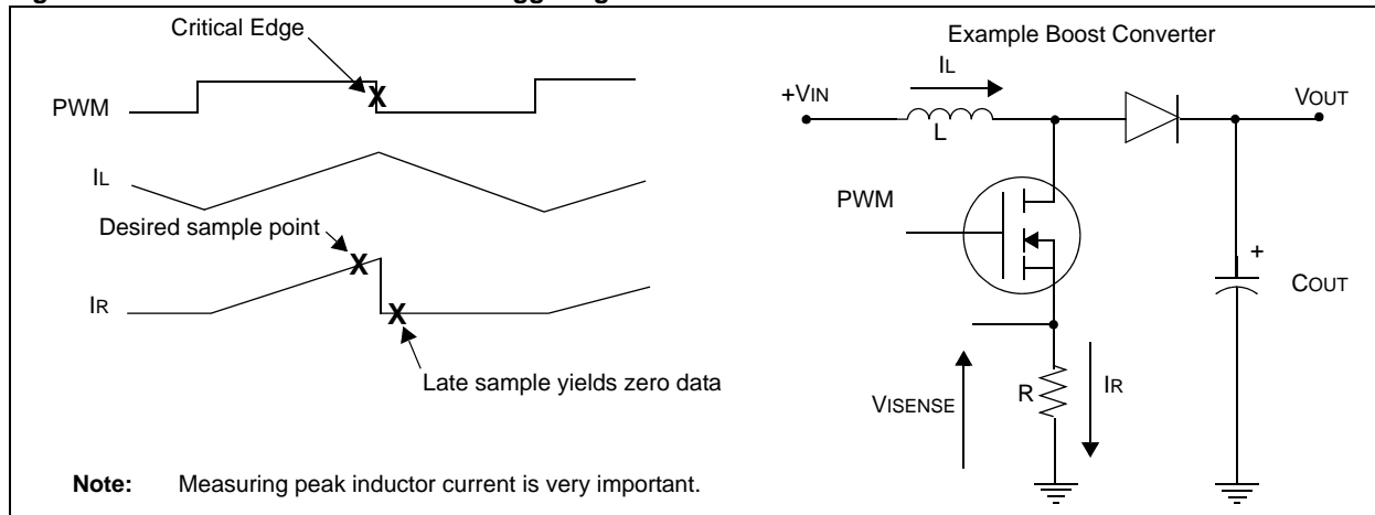
Figure 43-55: Need for Precise ADC Triggering
