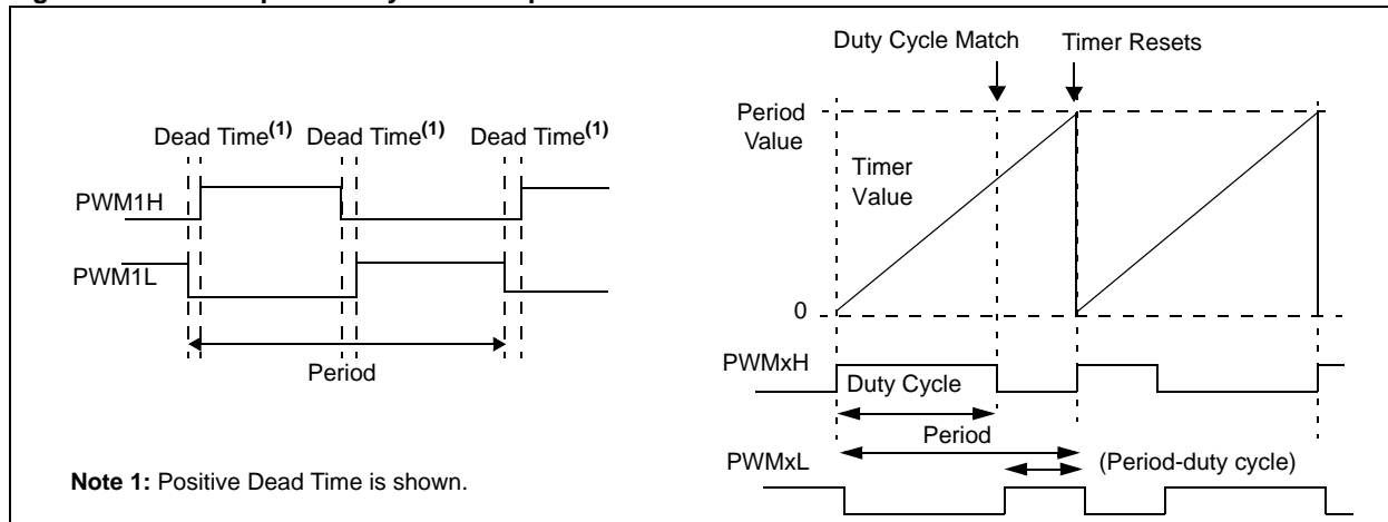
Figure 43-30: Complementary PWM Output Mode
