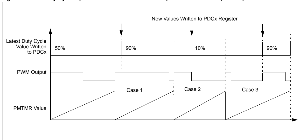
Figure 43-45: Duty Cycle Update Times When Immediate Updates are Enabled (IUE = 1)
