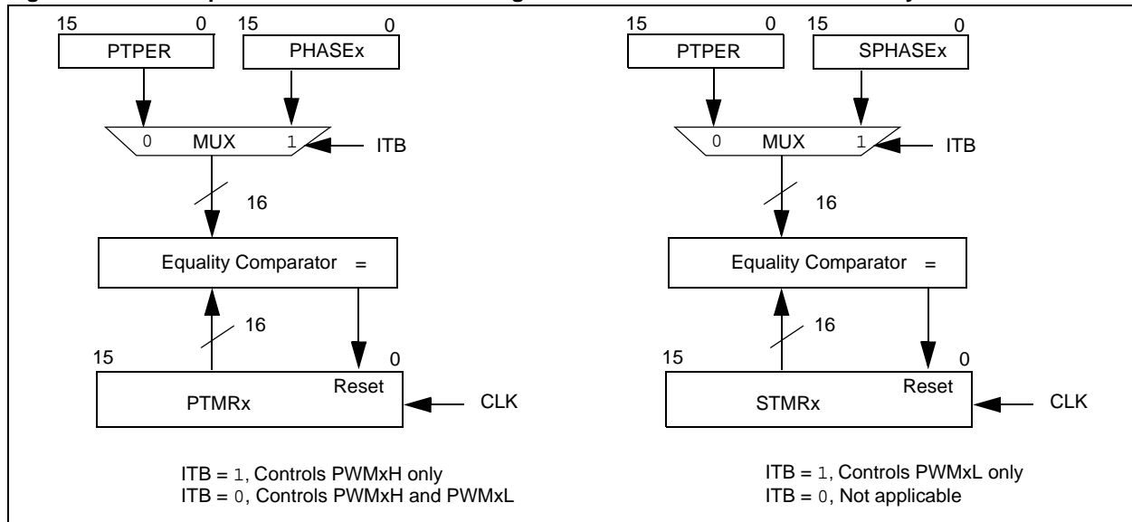
Figure 43-10: Independent Time Base Block Diagrams for Devices without a Secondary Master Time Base
