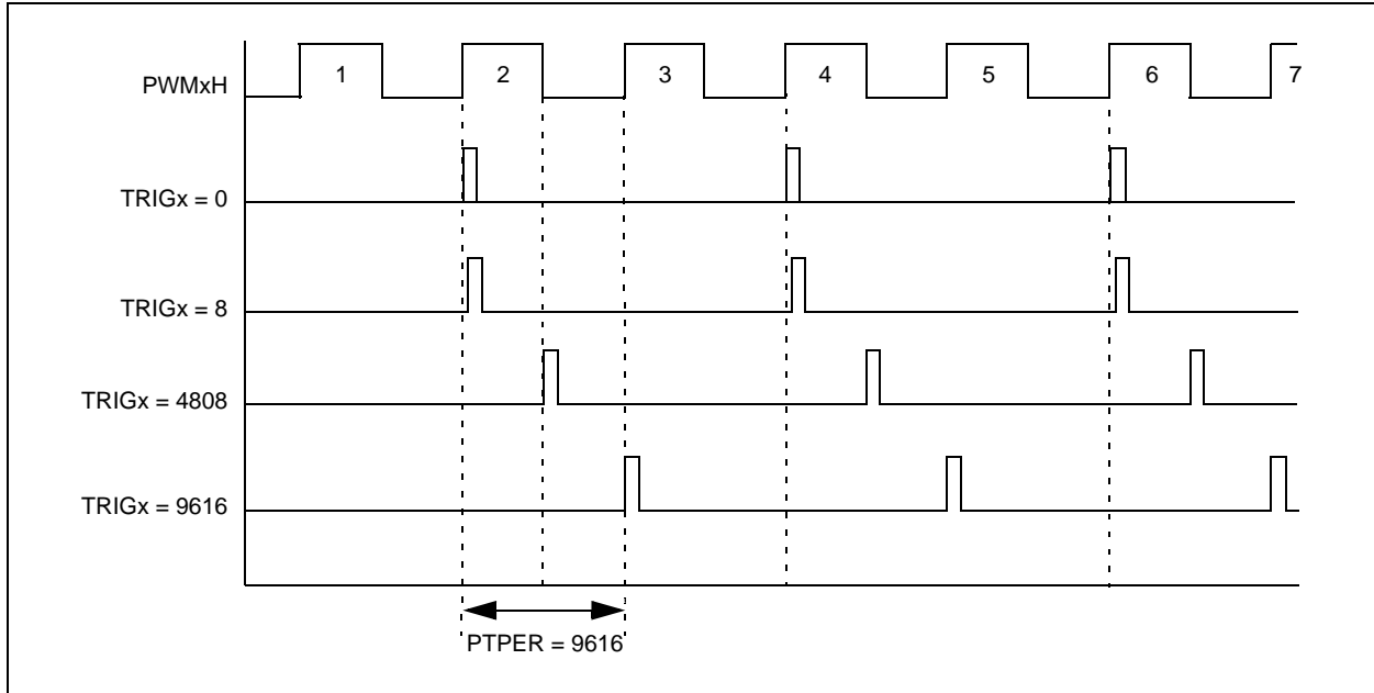
Figure 43-25: PWM Trigger Signal in Relation to the PWM Output (TRGDIV = 2, TRGSTRT = 0)
