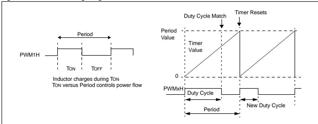
Figure 43-5: Standard Edge-Aligned PWM Mode
