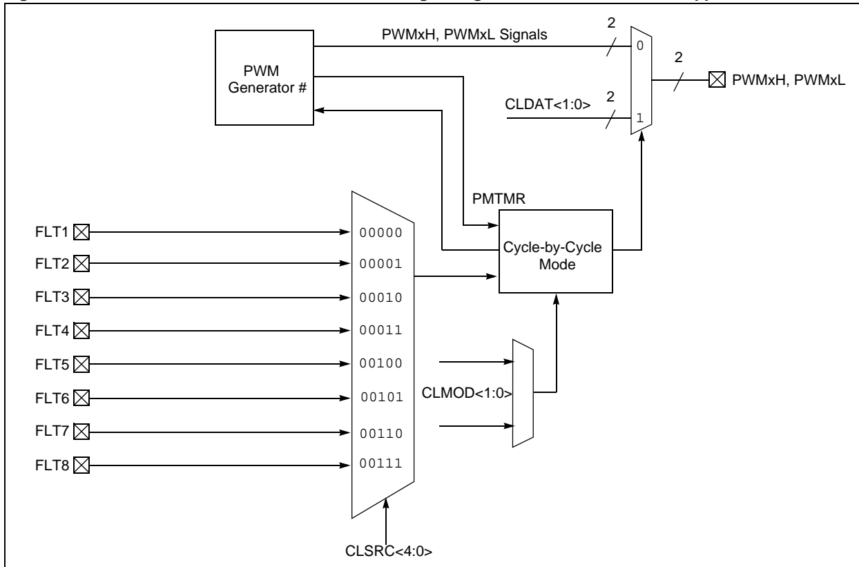
Figure 43-36: PWM Current-Limit Control Circuit Logic Diagram for Devices with Remappable I/O
