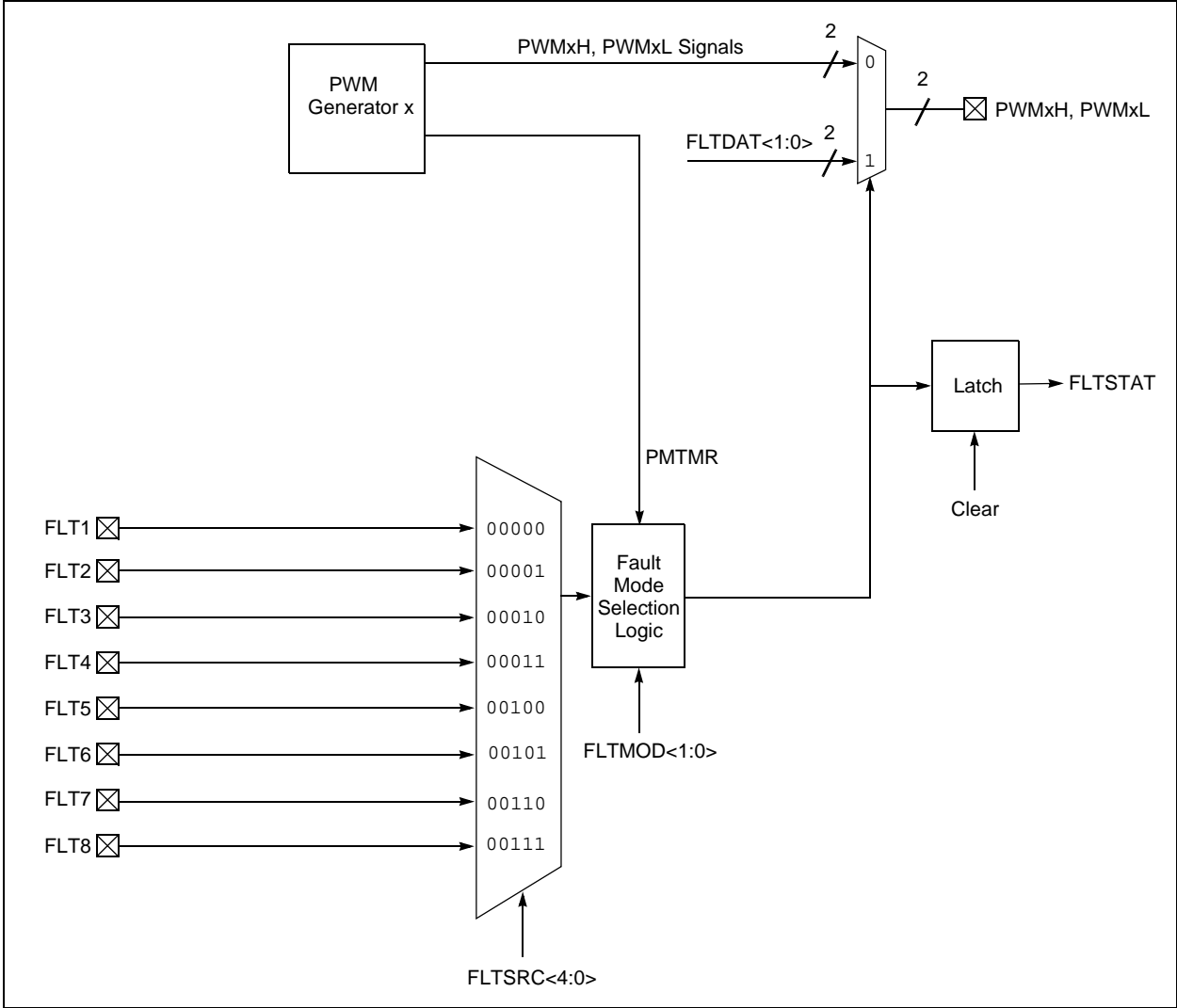
Figure 43-33: PWM Fault Control Module Block Diagram for Devices with Remappable I/O
