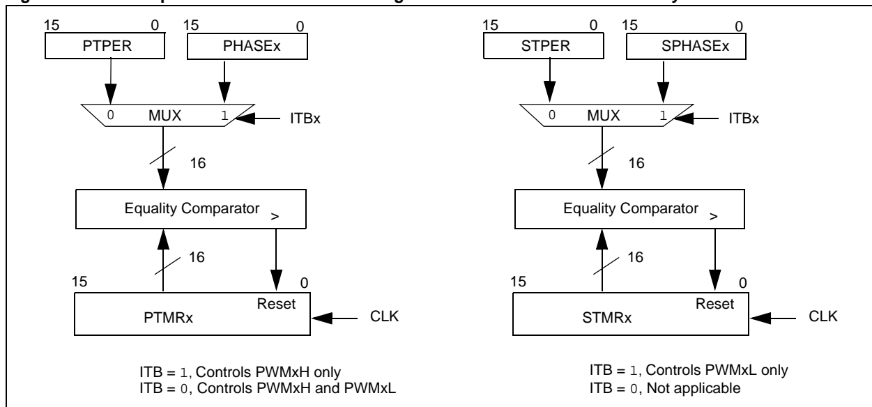
Figure 43-11: Independent Time Base Block Diagrams for Devices with a Secondary Master Time Base
