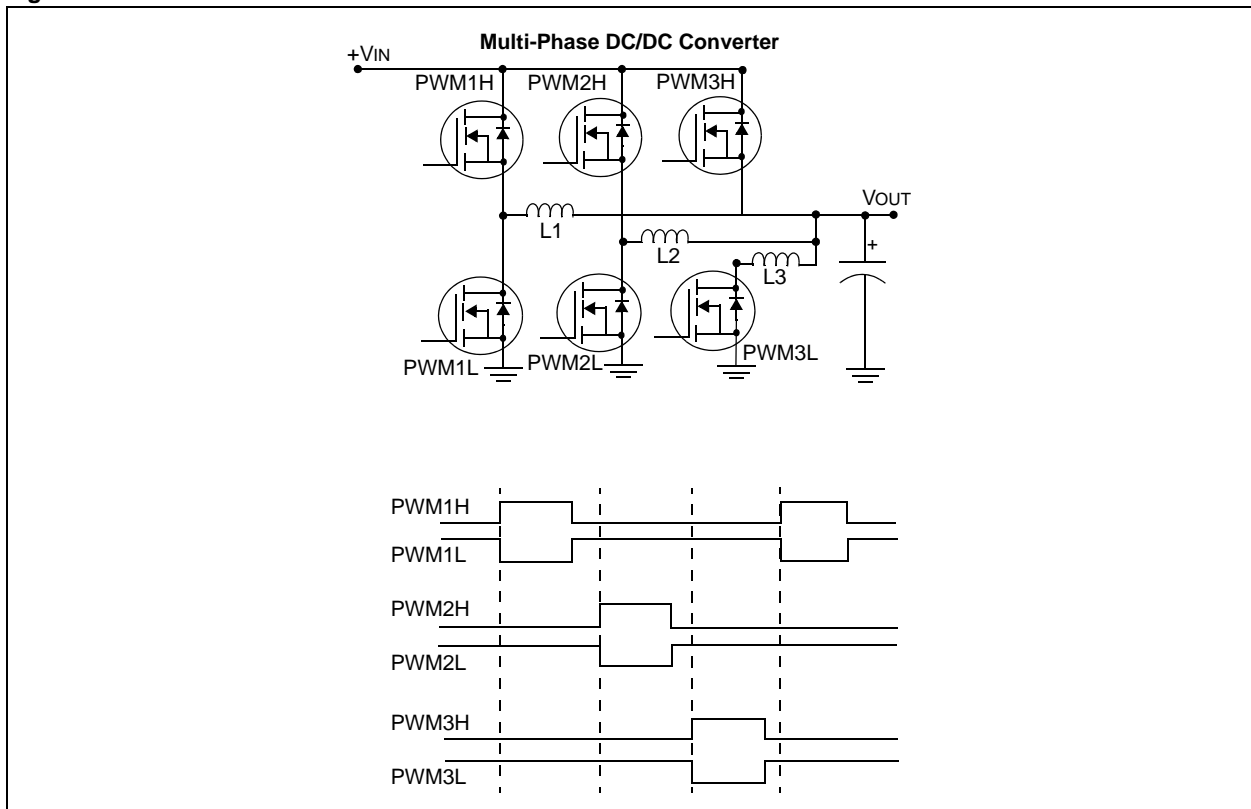
Figure 43-48: Multi-Phase PWM
