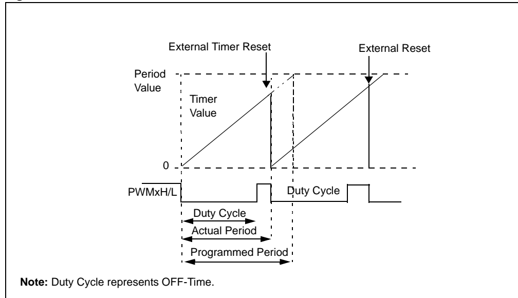
Figure 43-53: Constant Off-Time PWM
