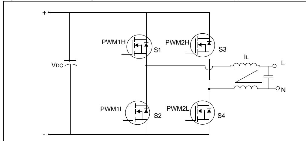
Figure 43-7: Center-Aligned PWM Mode in Power Inverter/UPS Applications
