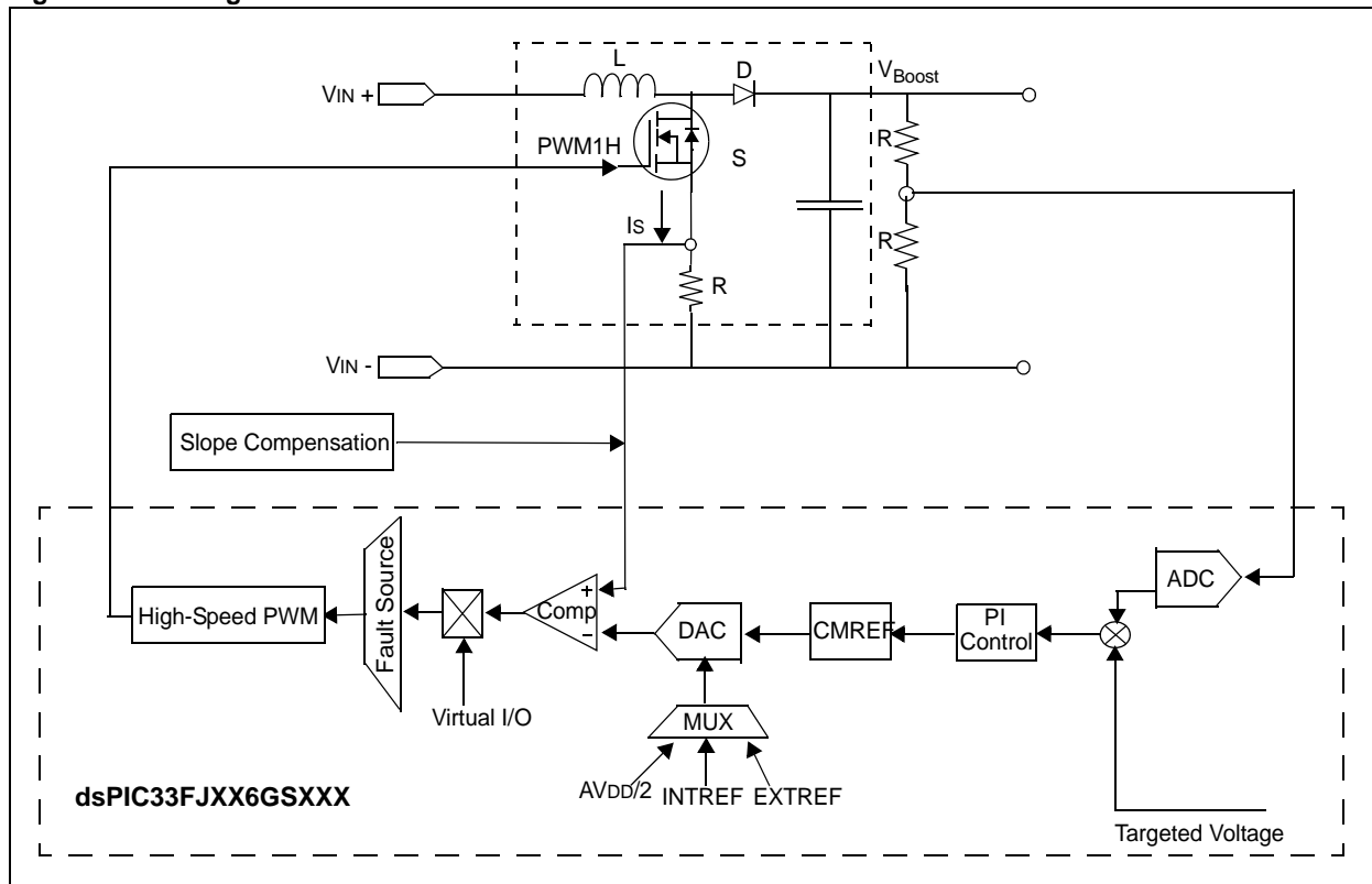
Figure 43-38: Digital Peak Current Mode Boost Converter
