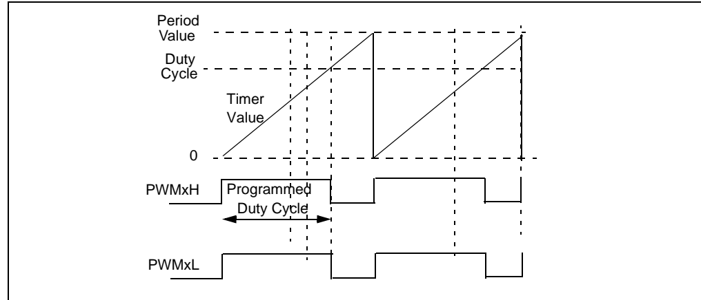
Figure 43-31: Redundant PWM Output Mode
