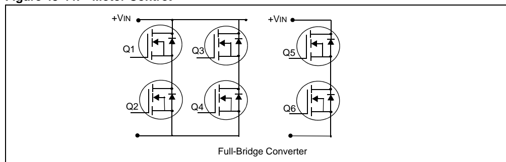
Figure 43-44: Motor Control
