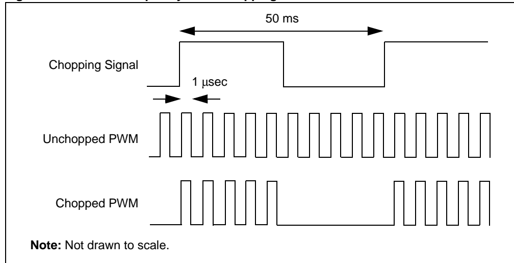
Figure 43-42: Low-Frequency PWM Chopping
