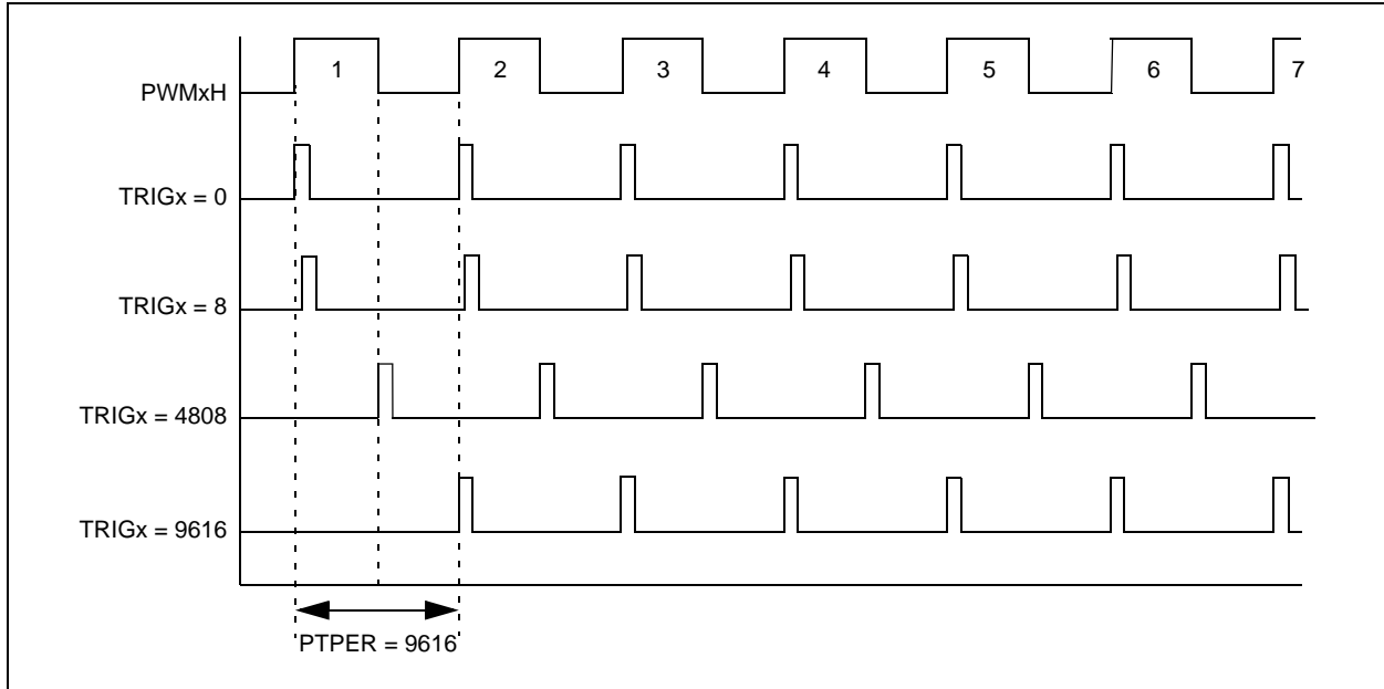
Figure 43-21: PWM Trigger Signal in Relation to the PWM Output (TRGDIV = 0, TRGSTRT = 1)
