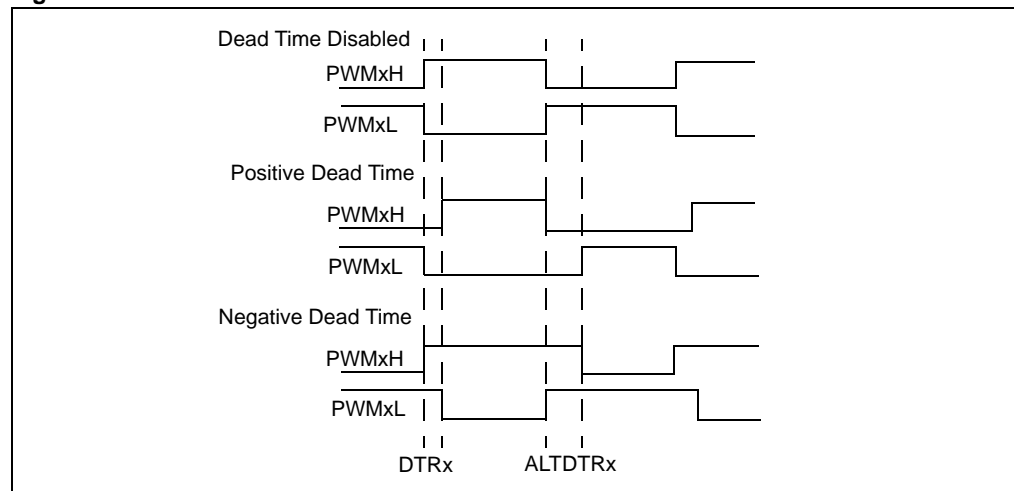
Figure 43-14: Dual Dead Time Waveforms
