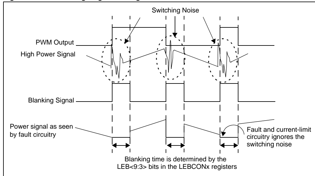
Figure 43-39: Leading-Edge Blanking
