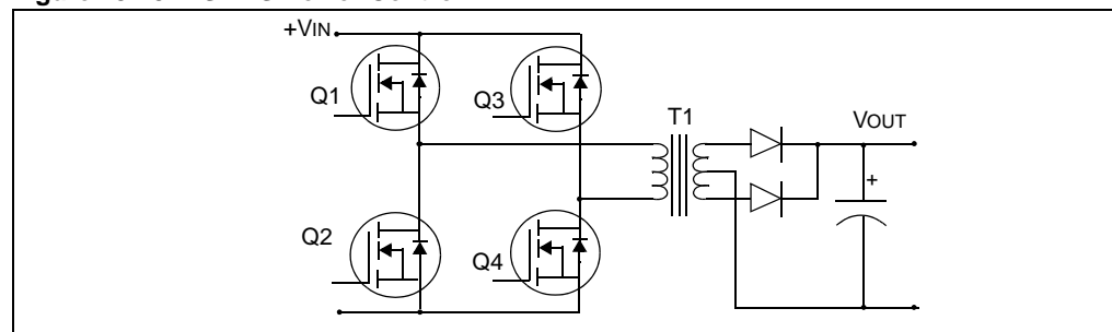
Figure 43-43: SMPS Power Control
