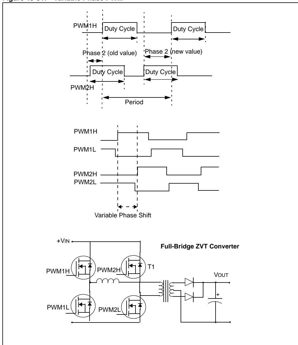
Figure 43-51: Variable Phase PWM
