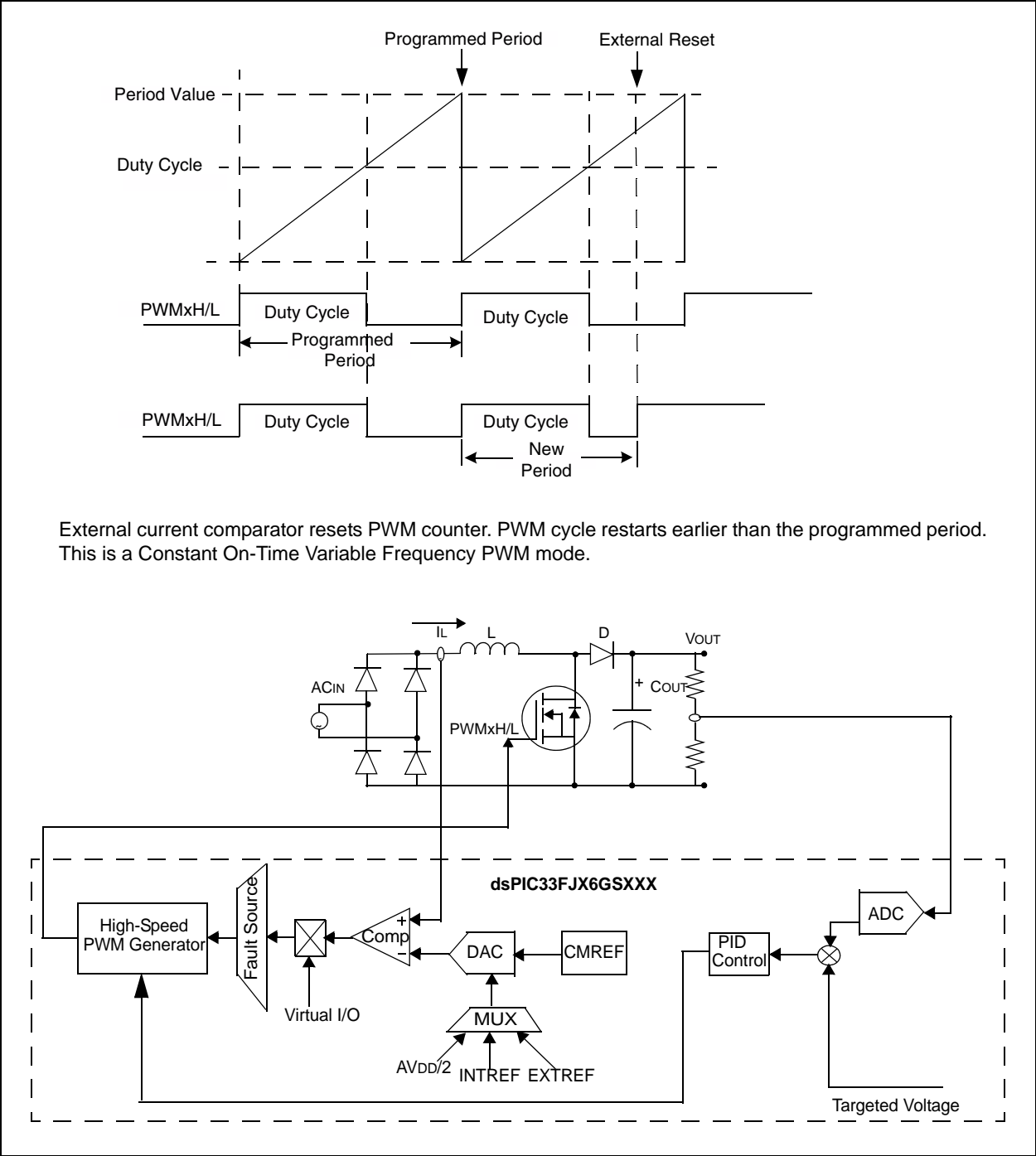
Figure 43-52: Current Reset PWM
