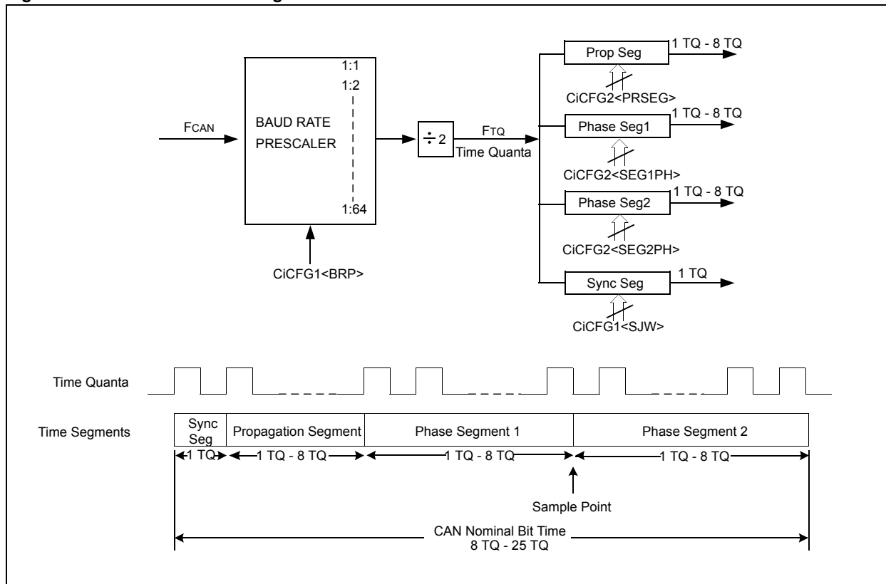
Figure 21-17: ECAN™ Bit Timing
