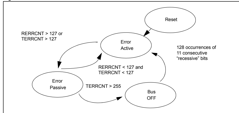
Figure 21-18: Error Modes
