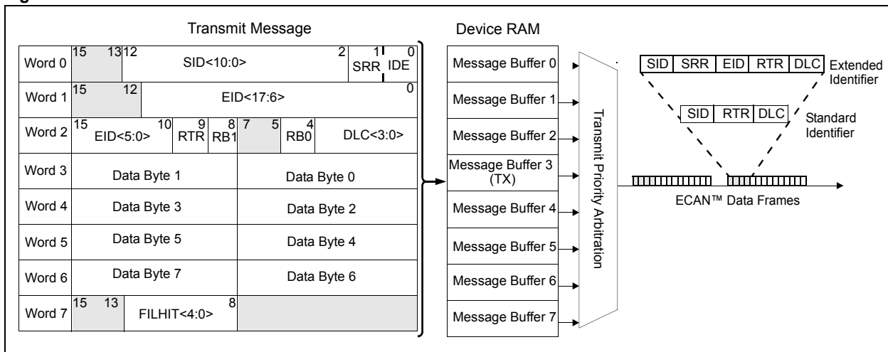
Figure 21-8: ECAN™ Transmission
