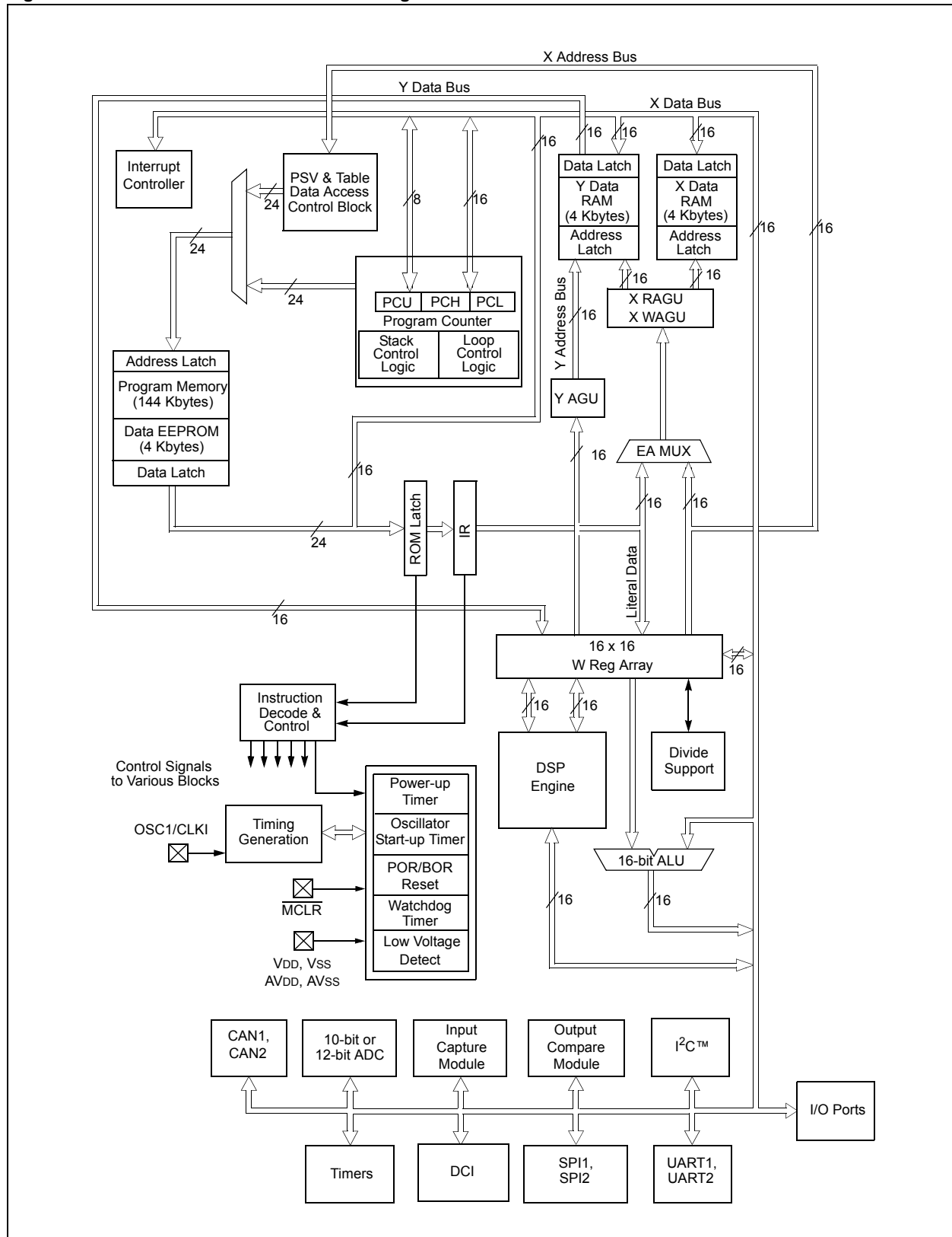
Figure 2-1: dsPIC30F CPU Core Block Diagram
