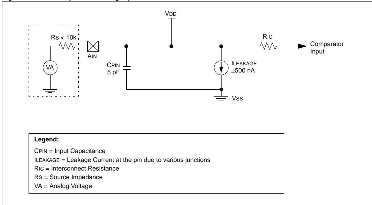
Figure 34-4: Comparator Analog Input Model
