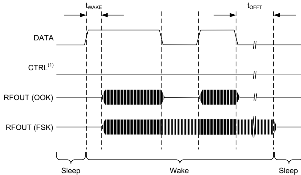
FIGURE 28-5: DATA PIN TRANSMIT TIMING DIAGRAM
