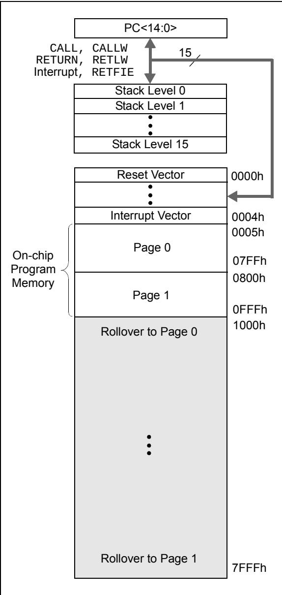
FIGURE 3-1: PROGRAM MEMORY MAP AND STACK FOR PIC12LF1840T39A
