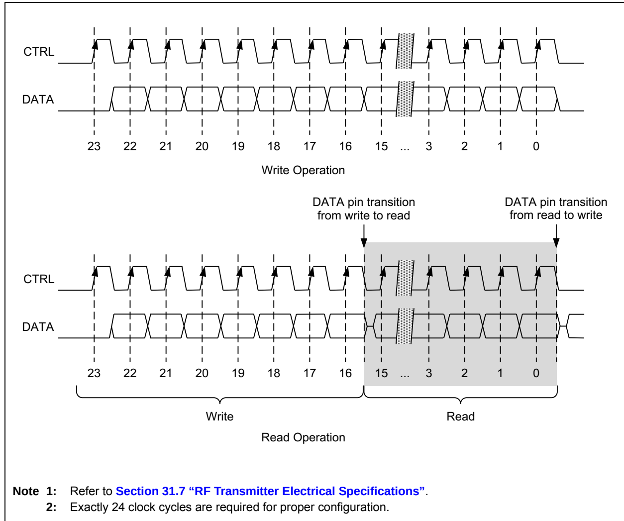
FIGURE 28-3: REGISTER WRITE AND READ OPERATIONS
