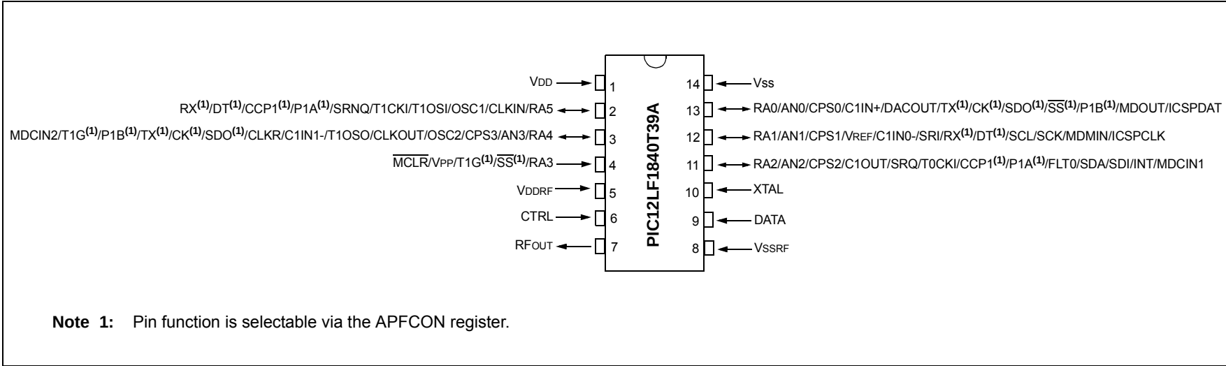
FIGURE 1: 14-PIN DIAGRAM, PIC12LF1840T39A (TSSOP)
