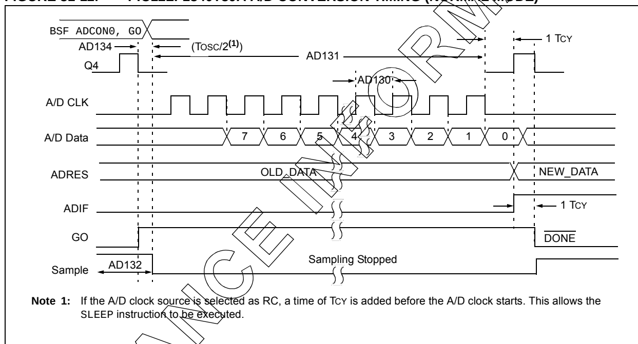
FIGURE 31-11: PIC12LF1840T39A A/D CONVERSION TIMING (NORMAL MODE)
