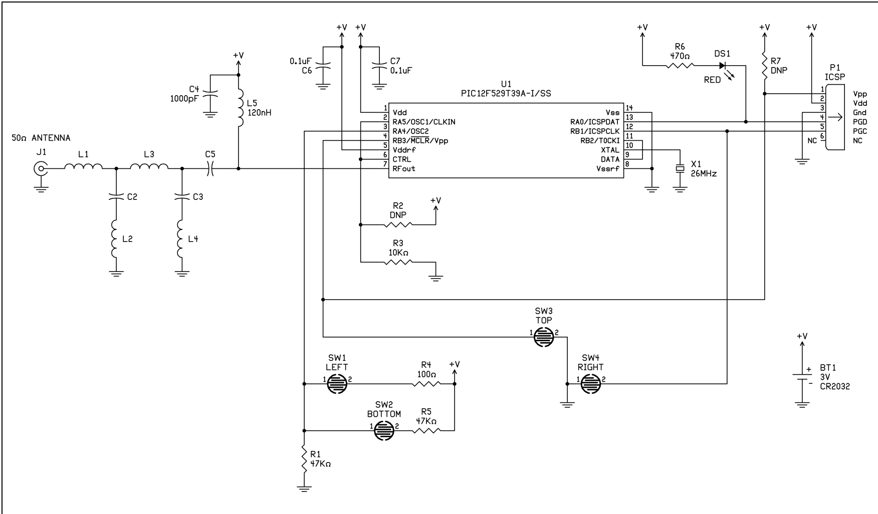
FIGURE 28-8: APPLICATION SCHEMATIC
