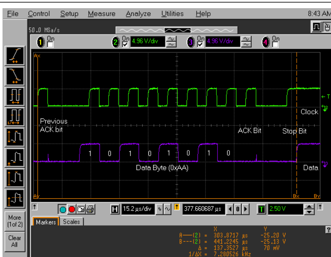
FIGURE 4: DATA BYTE AND STOP BIT
