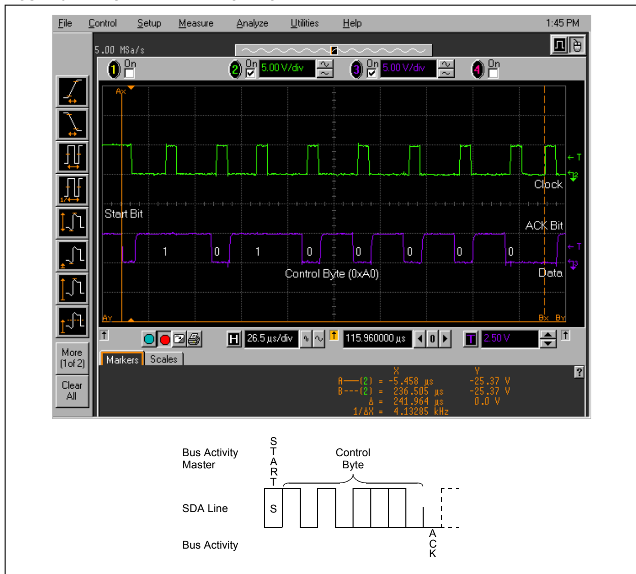
FIGURE 3: START BIT AND CONTROL BYTE
