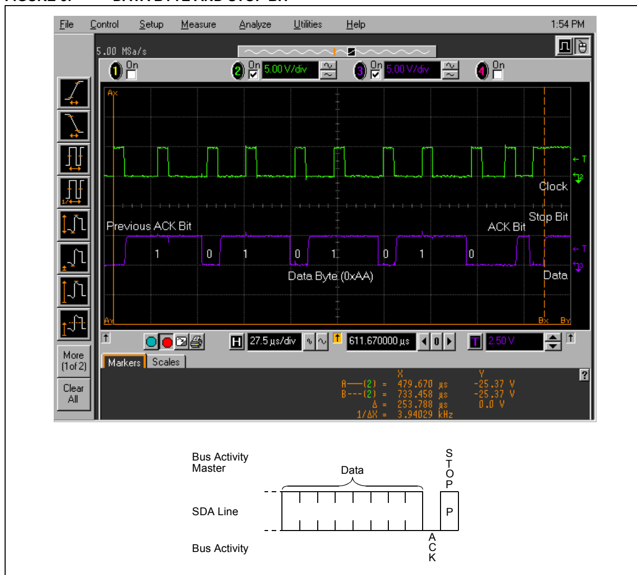
FIGURE 5: DATA BYTE AND STOP BIT
