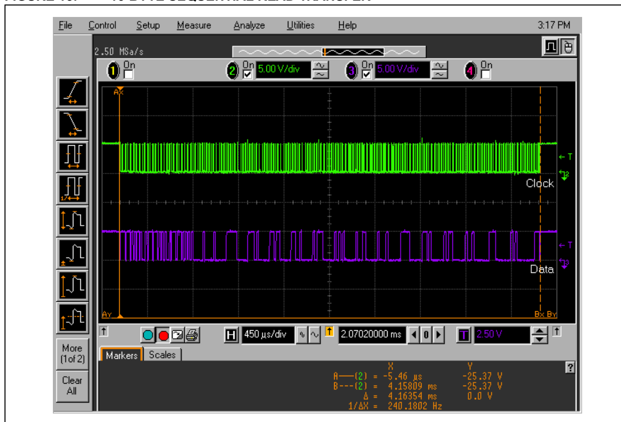
FIGURE 15: 16-BYTE SEQUENTIAL READ TRANSFER
