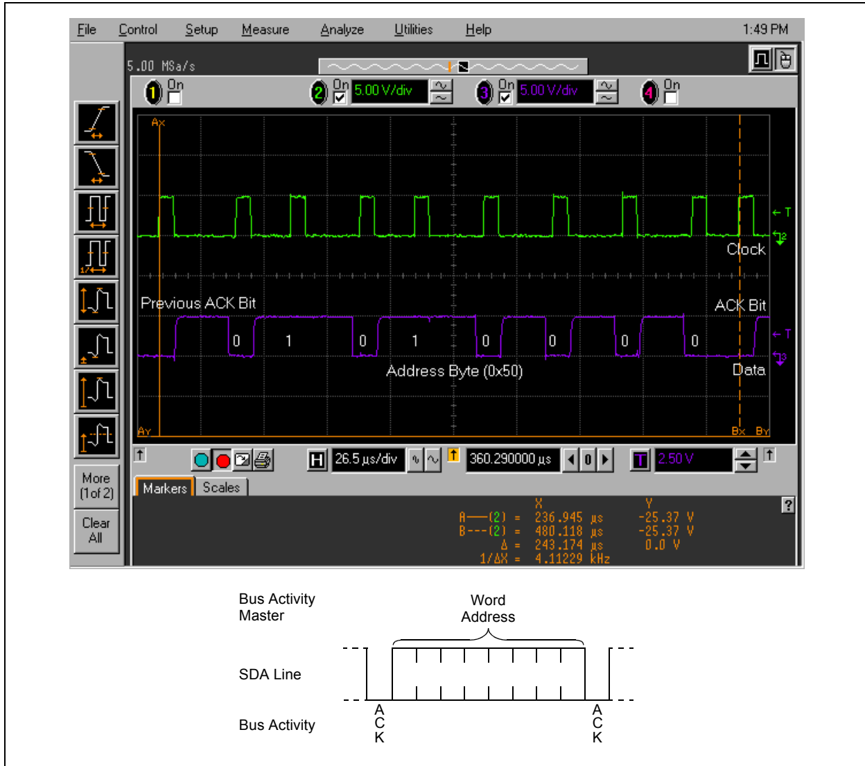
FIGURE 4: ADDRESS BYTE
