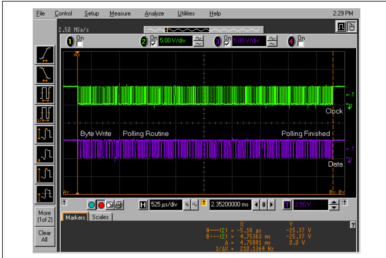
FIGURE 9: ENTIRE BYTE WRITE TRANSFER (1 BYTE, INCLUDES POLLING)
