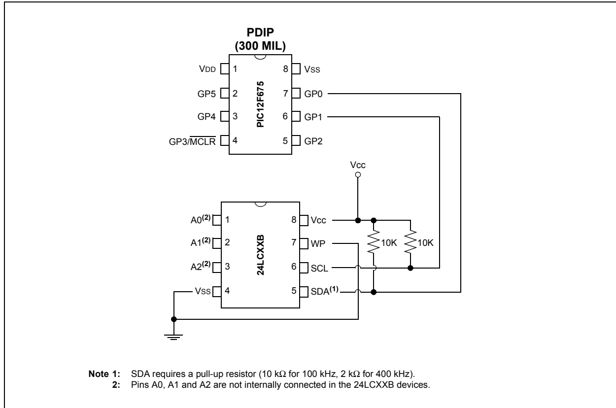
FIGURE 2: CIRCUIT FOR PIC12F675 AND 24LCXXB DEVICES
