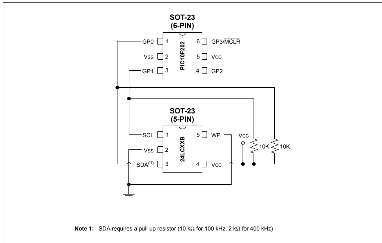
FIGURE 1: CIRCUIT FOR PIC10F202 AND 24LCXXB DEVICES
