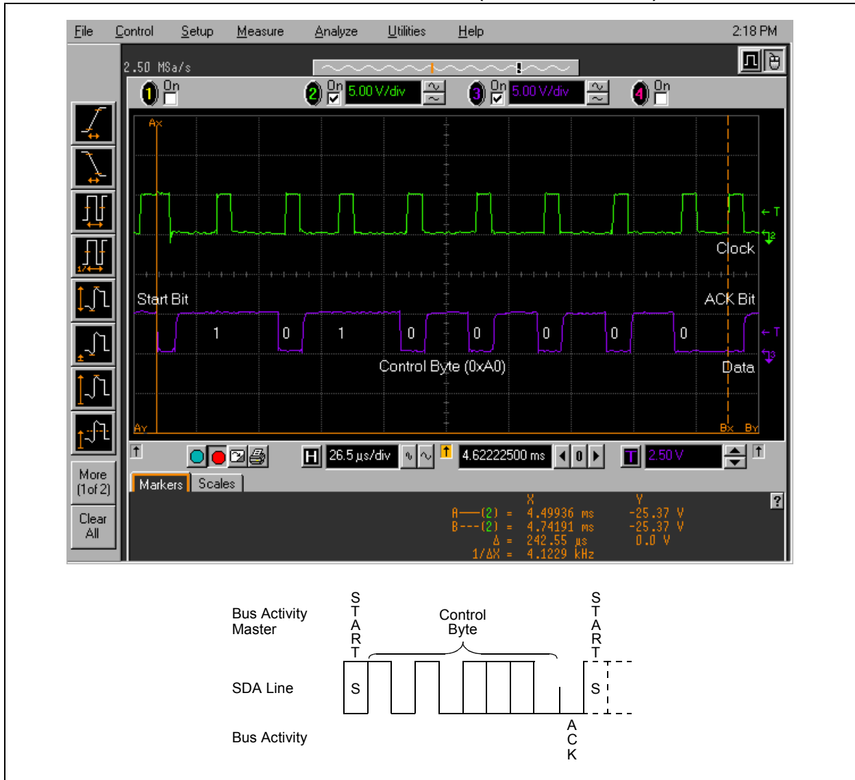
FIGURE 8: ACKNOWLEDGE POLLING FINISHED (SHOWING ACK BIT)
