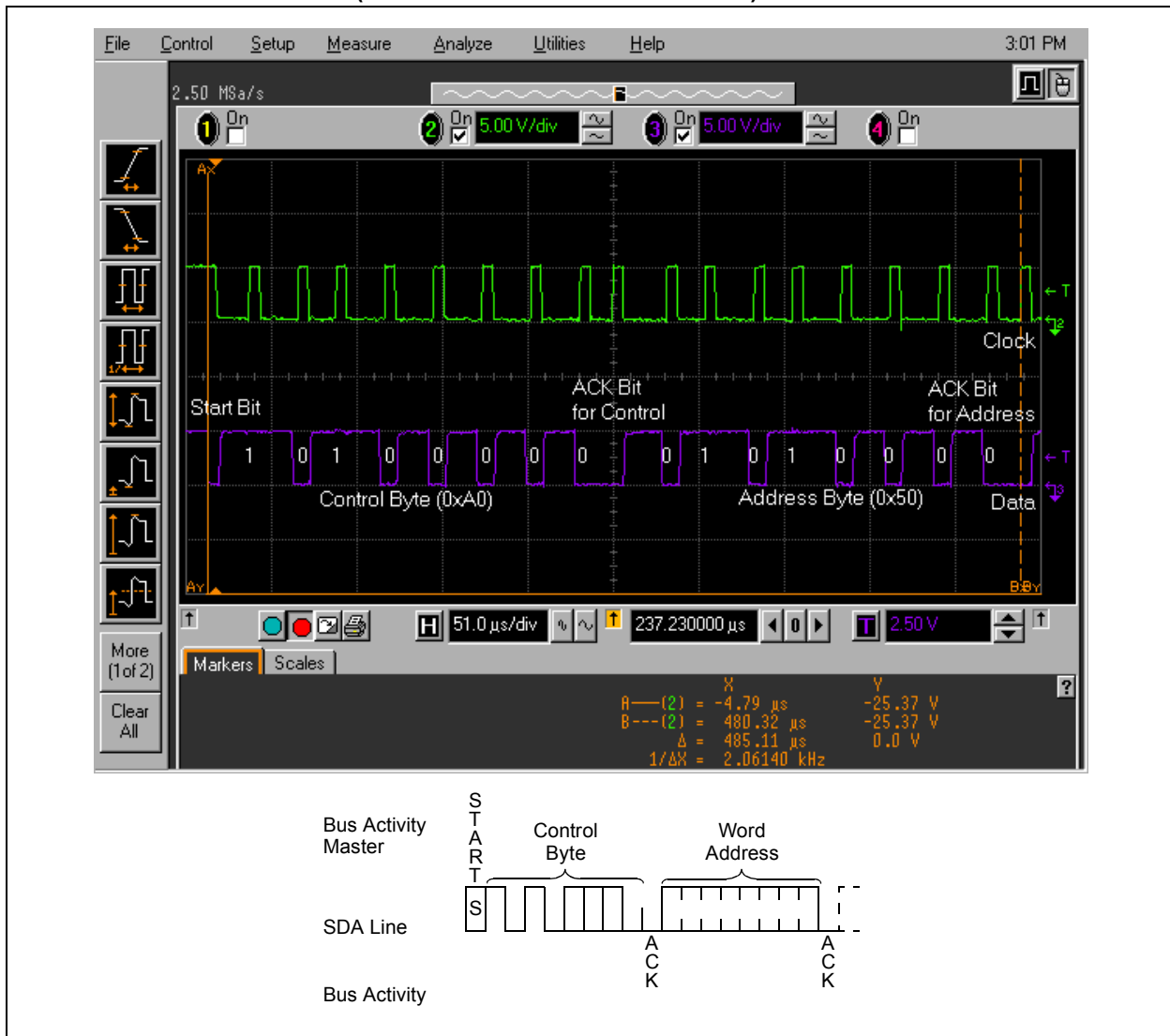
FIGURE 12: BYTE READ (CONTROL BYTE AND ADDRESS)
