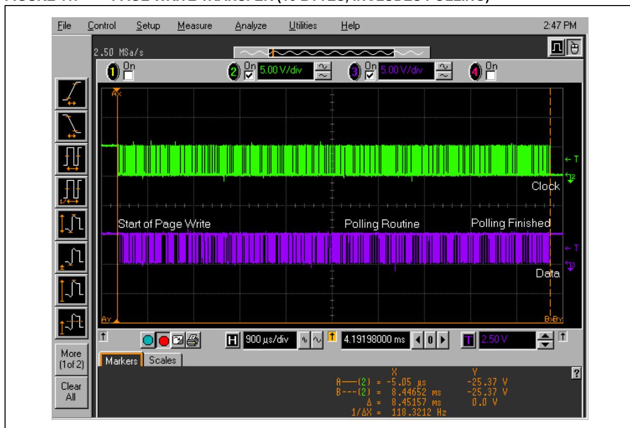
FIGURE 11: PAGE WRITE TRANSFER (16 BYTES, INCLUDES POLLING)
