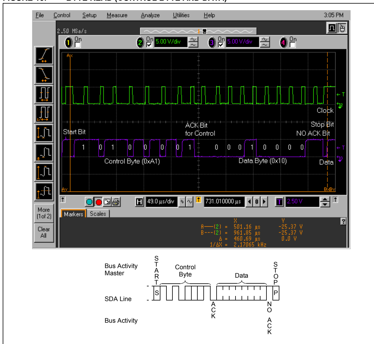
FIGURE 13: BYTE READ (CONTROL BYTE AND DATA)
