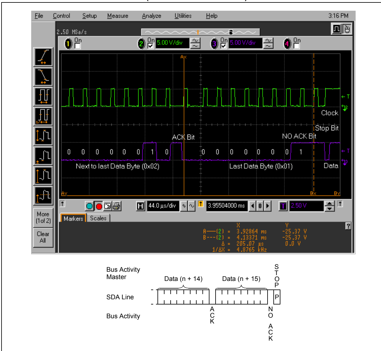
FIGURE 14: SEQUENTIAL READ (LAST TWO DATA BYTES)
