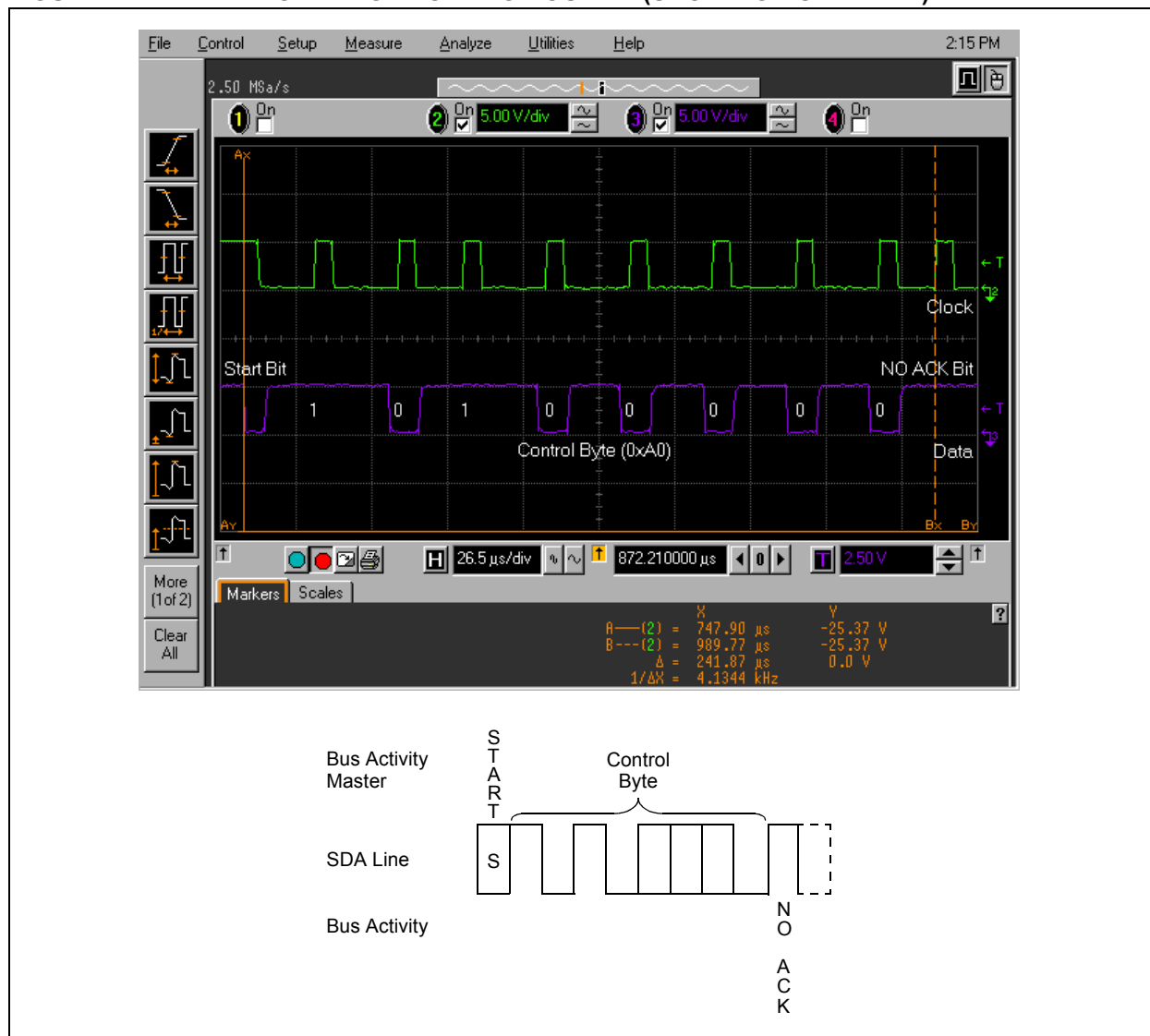
FIGURE 7: ACKNOWLEDGE POLLING ROUTINE (SHOWING NO ACK BIT)
