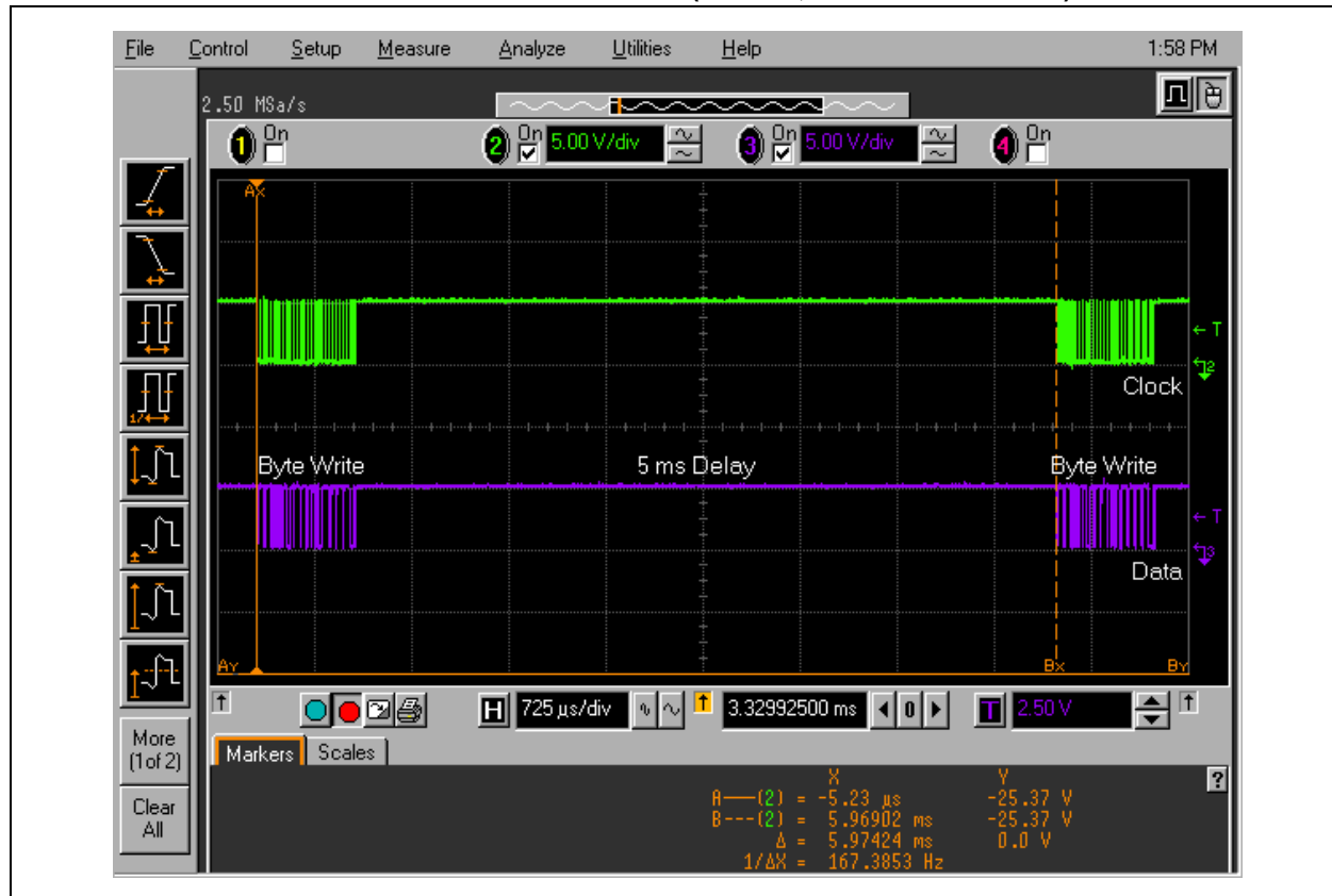
FIGURE 6: ENTIRE BYTE WRITE TRANSFER (1 BYTE, INCLUDES DELAY)
