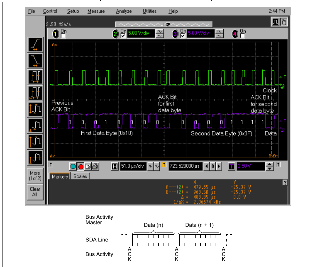
FIGURE 10: PAGE WRITE (TWO CONSECUTIVE DATA BYTES)
