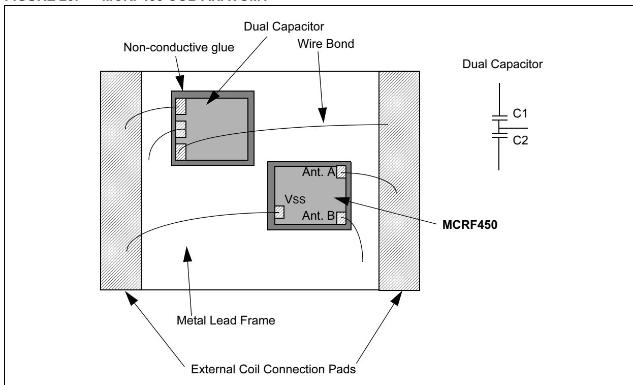
FIGURE 20: MCRF450 COB ANATOMY
