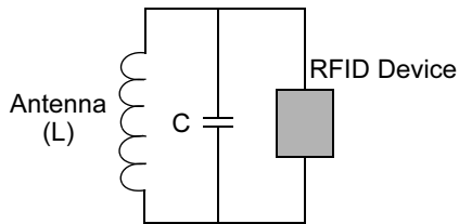
a) Configuration for 125 kHz RFID devices ( MCRF200 and MCRF250 )
