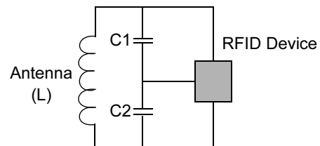
f) Configuration for 13.56 MHz RFID devices with no internal resonant capacitor. C1, C2 and L are external components. ( MCRF355 and MCRF450 )
