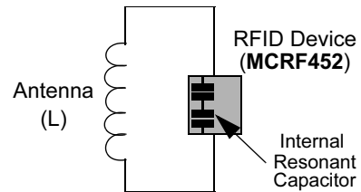
b) Configuration for MCRF452 .
