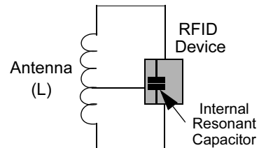
d) Configuration for 13.56 MHz RFID devices with internal resonant capacitor. ( MCRF360/ MCRF451/455 )
