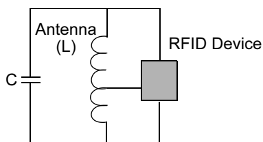
e) Configuration for 13.56 MHz RFID devices with no internal resonant capacitor ( MCRF355 and MCRF450 )
