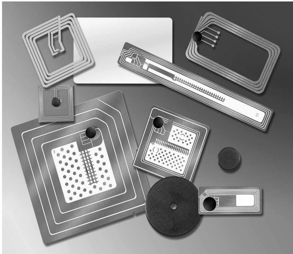
FIGURE 16: EXAMPLE OF VARIOUS 13.56 MHZ RFID TAGS
