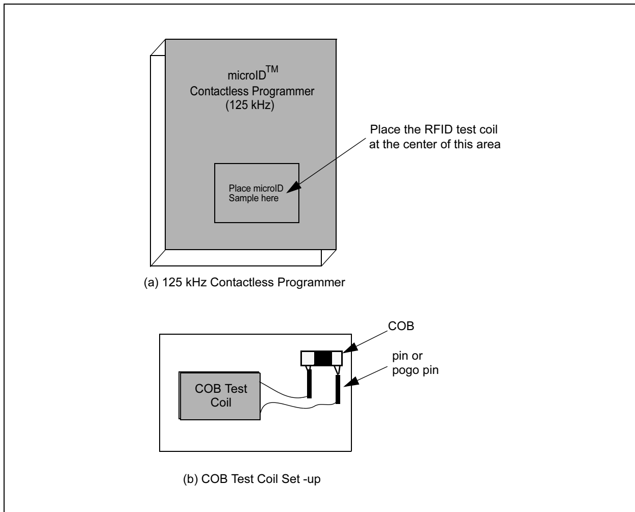
FIGURE 21: 125 KHZ CONTACTLESS PROGRAMMER AND COB TEST SET-UP
