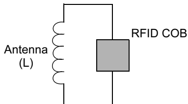
c) Configuration for COB ( MCRF200/250 , MCRF355 , MCRF450 , MCRF452 )
