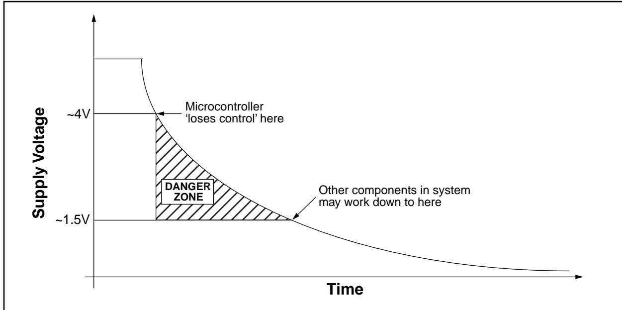
FIGURE 3: MICROCONTROLLER LOSES CONTROL WITH SLOWLY DECAYING SUPPLY
