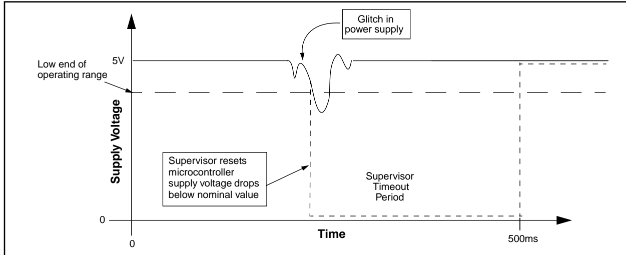
FIGURE 2: BROWN-OUT CONDITION
