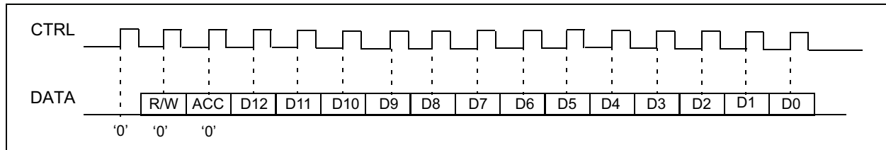
FIGURE 1: CONFIGURATION REGISTER WRITE
