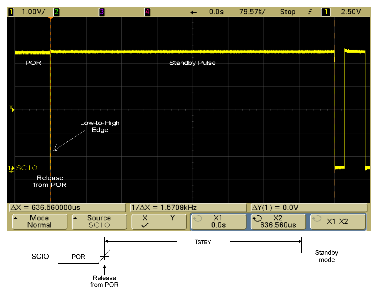
FIGURE 3: STANDBY PULSE
