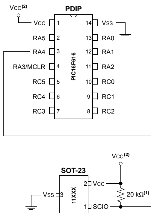
FIGURE 2: CIRCUIT FOR PIC16F616 AND 11XXX SERIAL EEPROM
