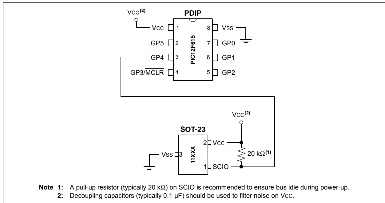
FIGURE 1: CIRCUIT FOR PIC12F615 AND 11XXX SERIAL EEPROM
