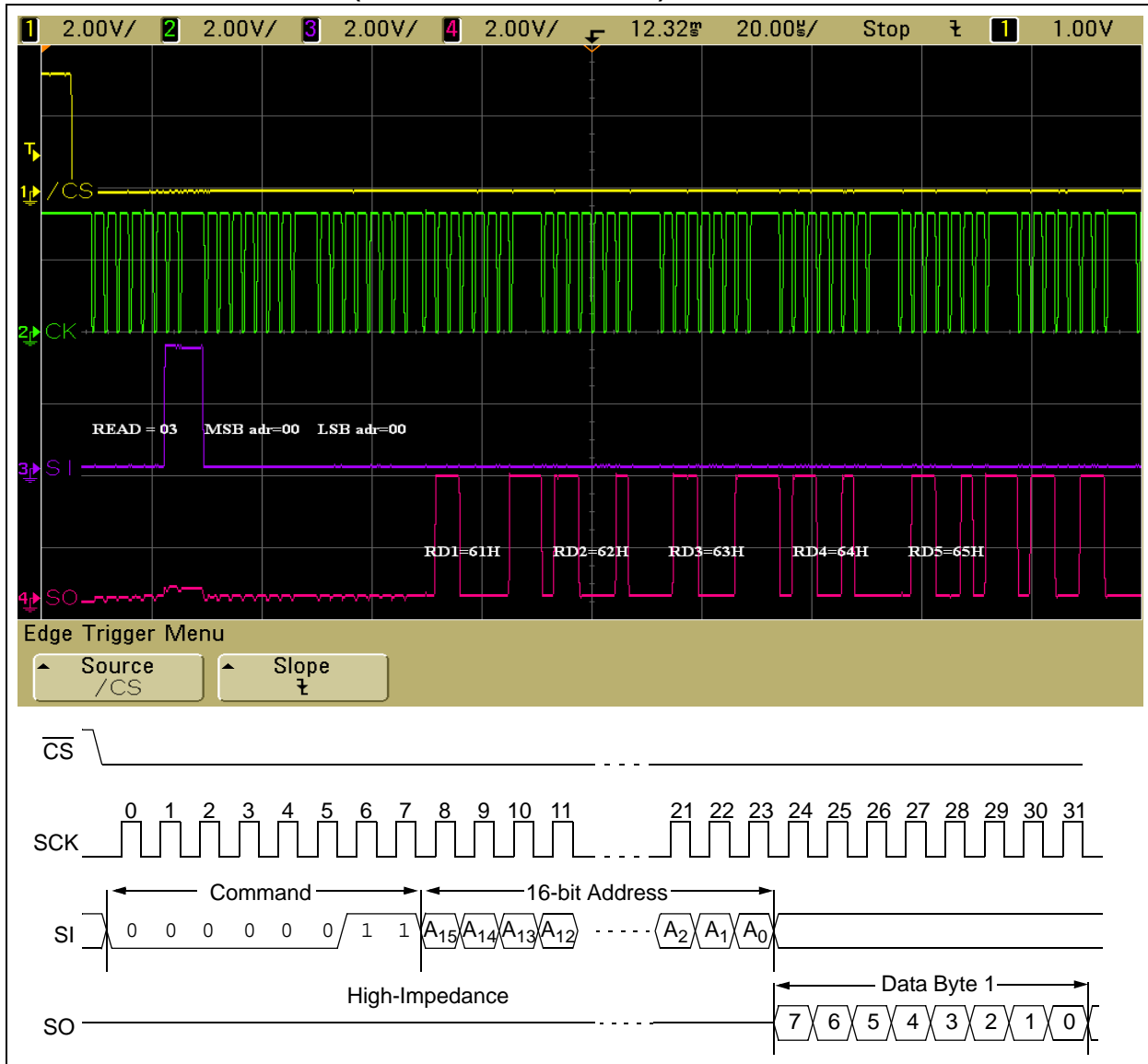
FIGURE 7: PAGE READ (FIRST FIVE READ BYTES)
