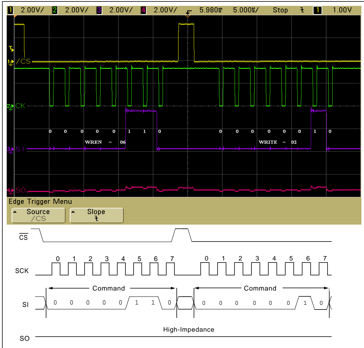
FIGURE 3: WRITE ENABLE AND WRITE COMMANDS
