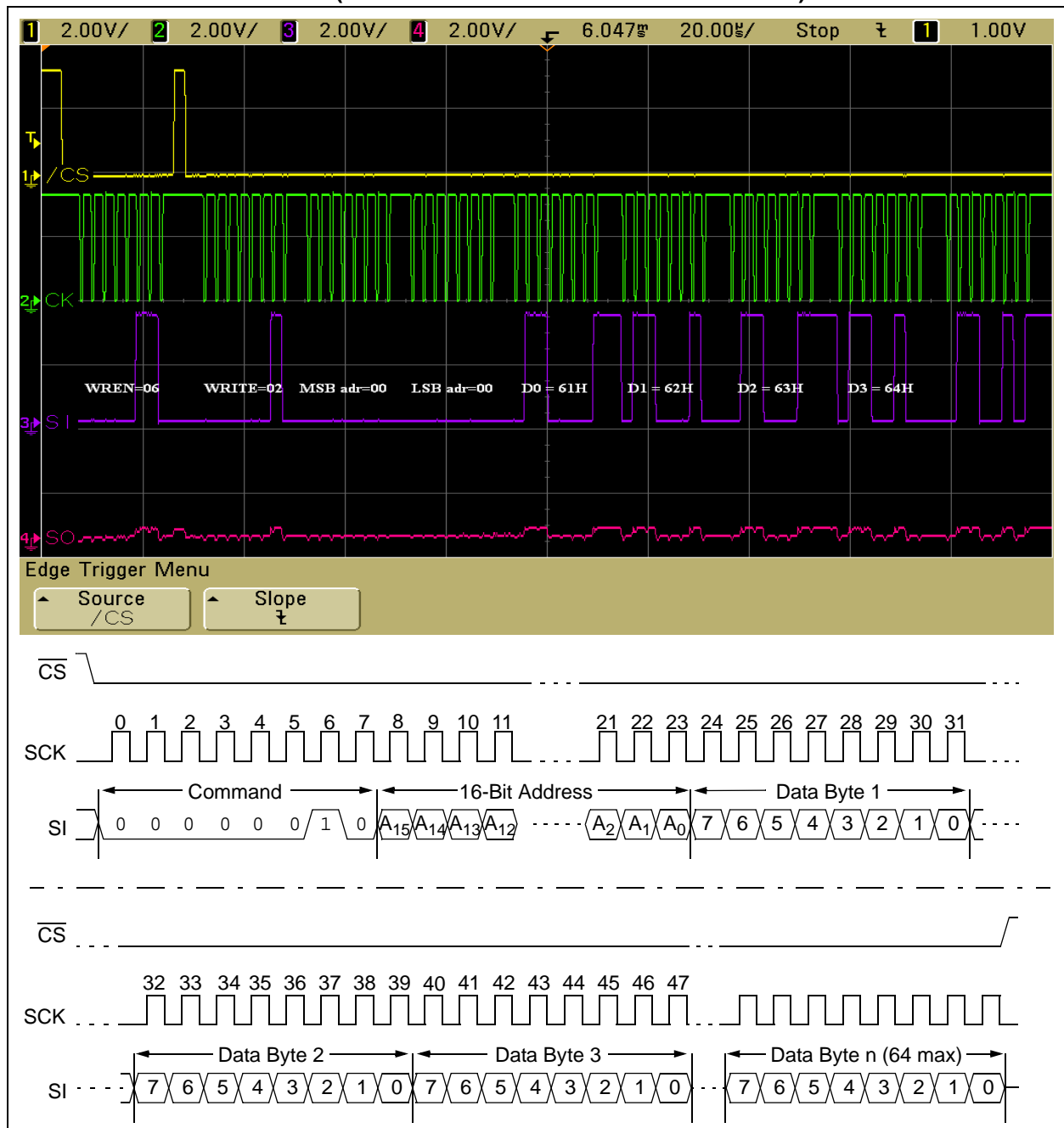
FIGURE 6: PAGE WRITE (FIRST FOUR CONSECUTIVE DATA BYTES)
