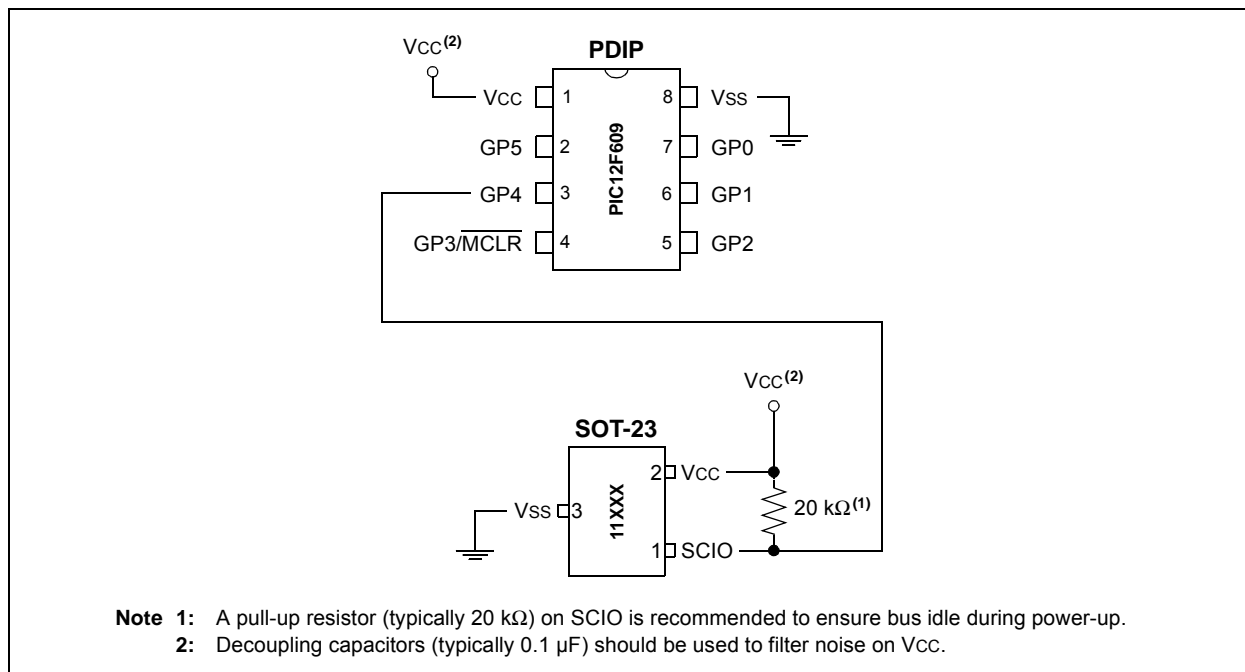
FIGURE 1: CIRCUIT FOR PIC12F609 AND 11XXX SERIAL EEPROM
