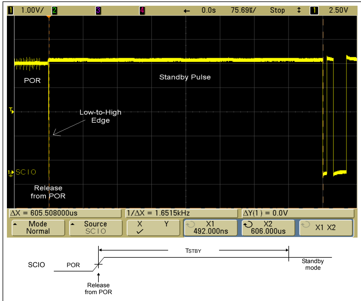
FIGURE 4: STANDBY PULSE
