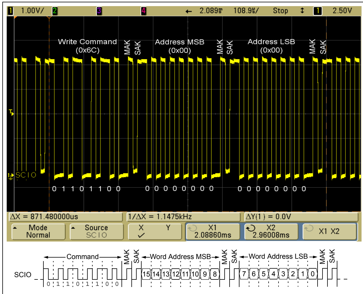
FIGURE 7: WRITE COMMAND AND WORD ADDRESS
