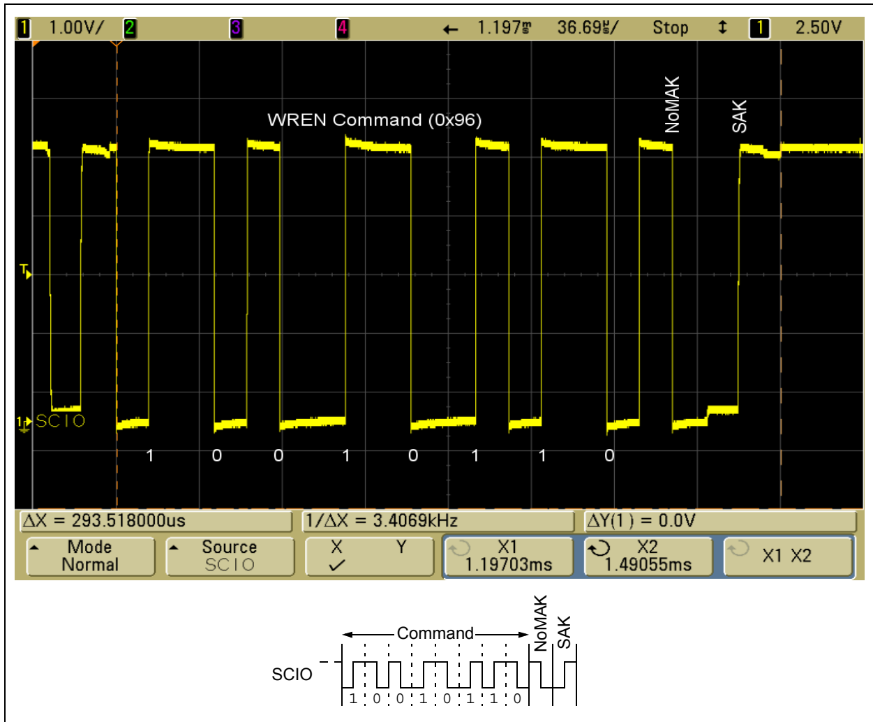
FIGURE 6: WRITE ENABLE COMMAND
