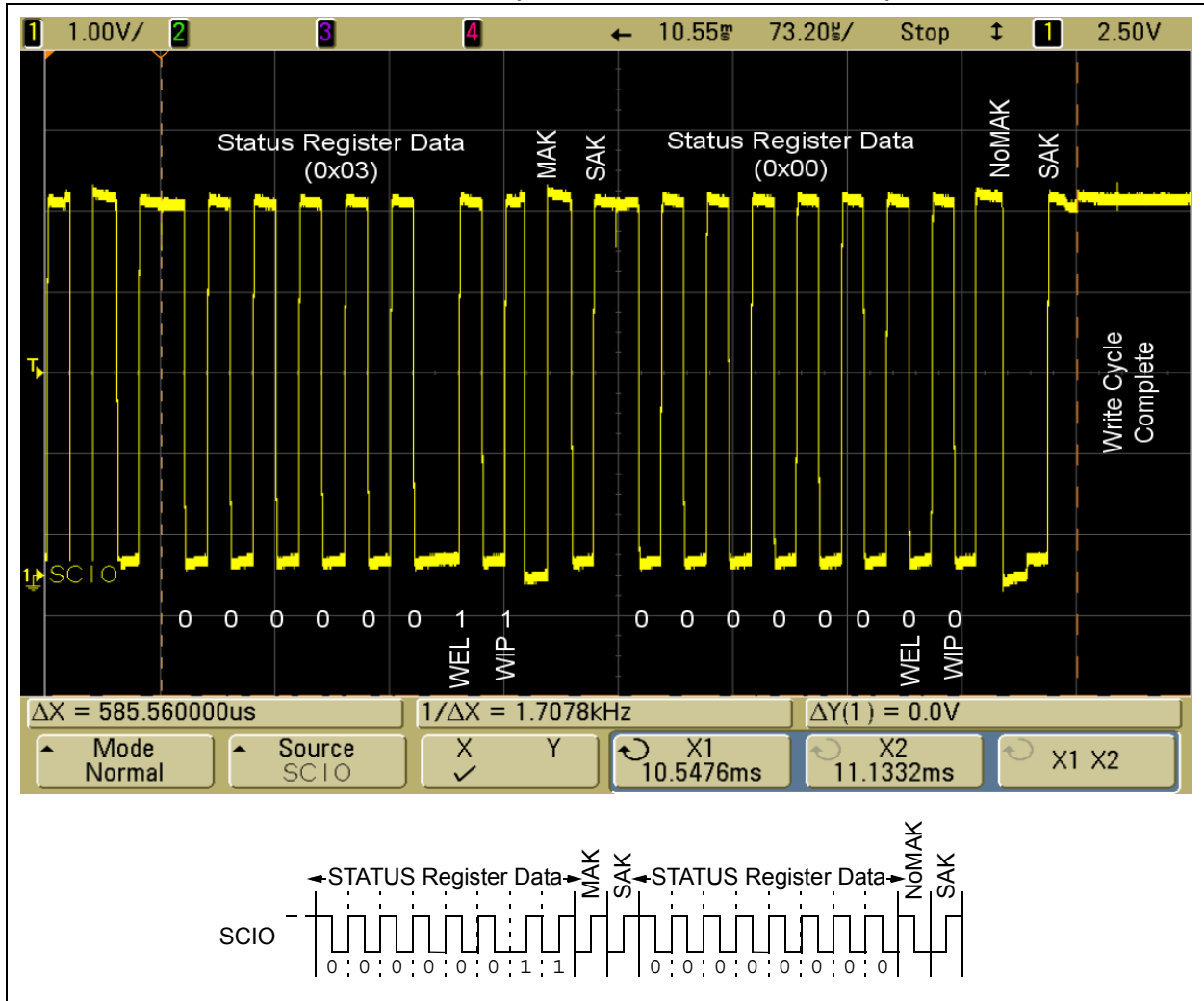
FIGURE 10: WIP POLLING FINISHED (SHOWING WRITE COMPLETE)
