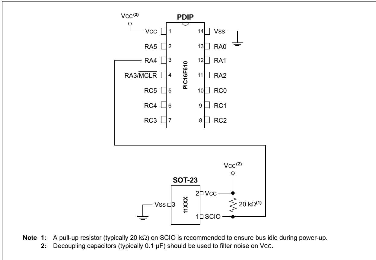
FIGURE 2: CIRCUIT FOR PIC16F610 AND 11XXX SERIAL EEPROM
