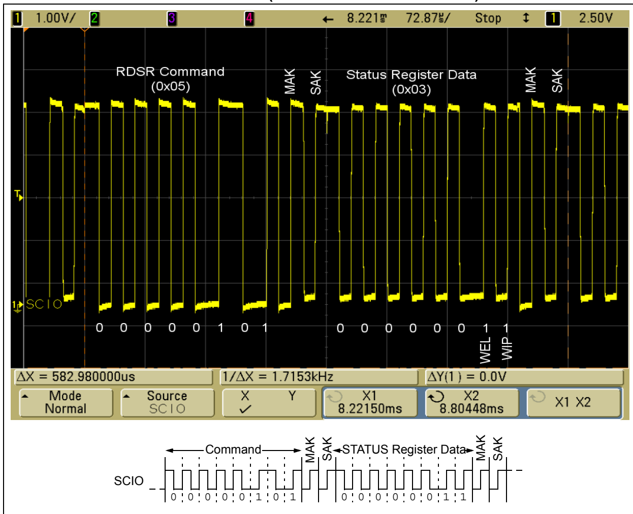
FIGURE 9: WIP POLLING ROUTINE (SHOWING WRITE-IN-PROCESS)
