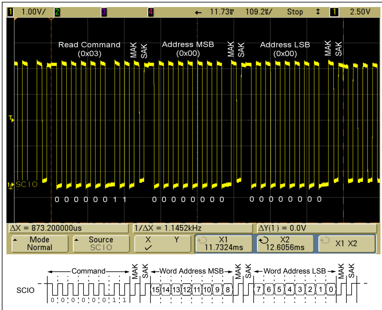
FIGURE 11: READ – COMMAND BYTE AND WORD ADDRESS
