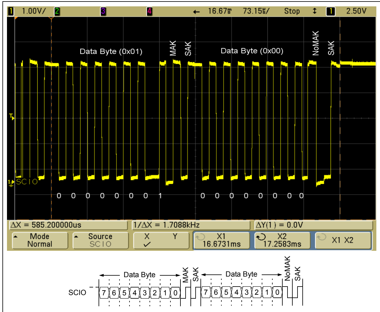
FIGURE 12: READ – FINAL TWO DATA BYTES
