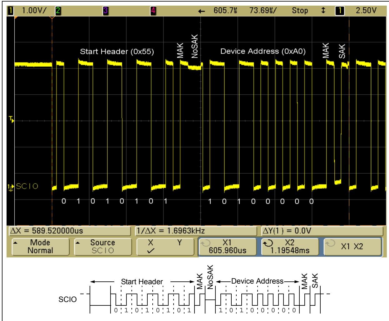
FIGURE 5: START HEADER AND DEVICE ADDRESS
