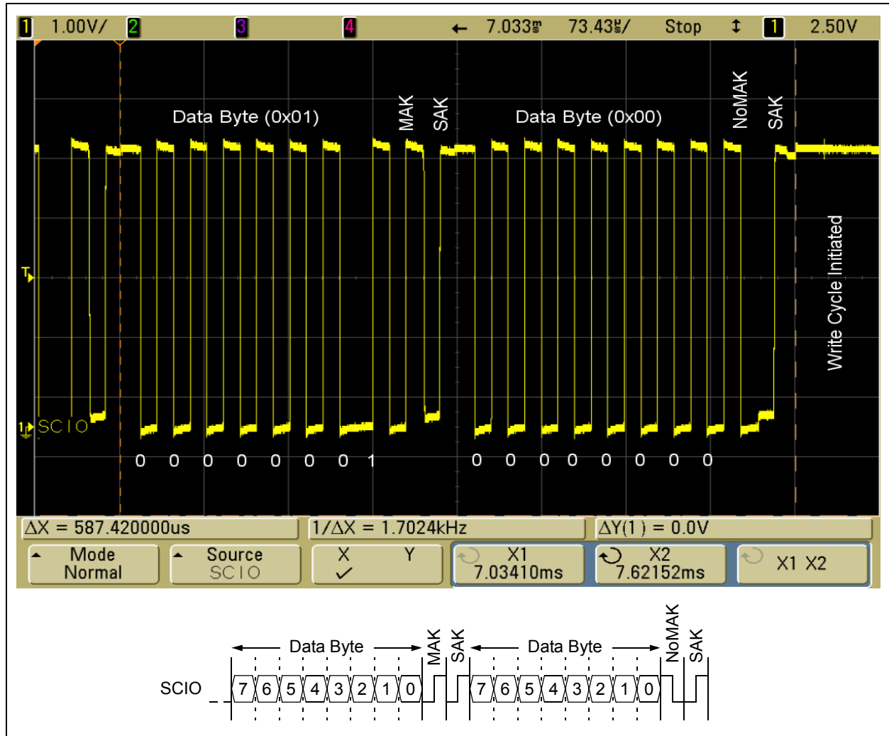
FIGURE 8: WRITE COMMAND FINAL TWO DATA BYTES
