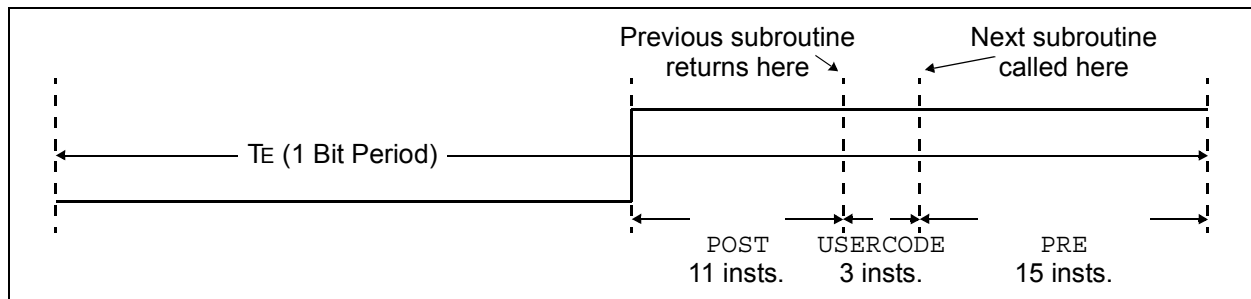
FIGURE 3: SUBROUTINE OVERHEAD TIMING
