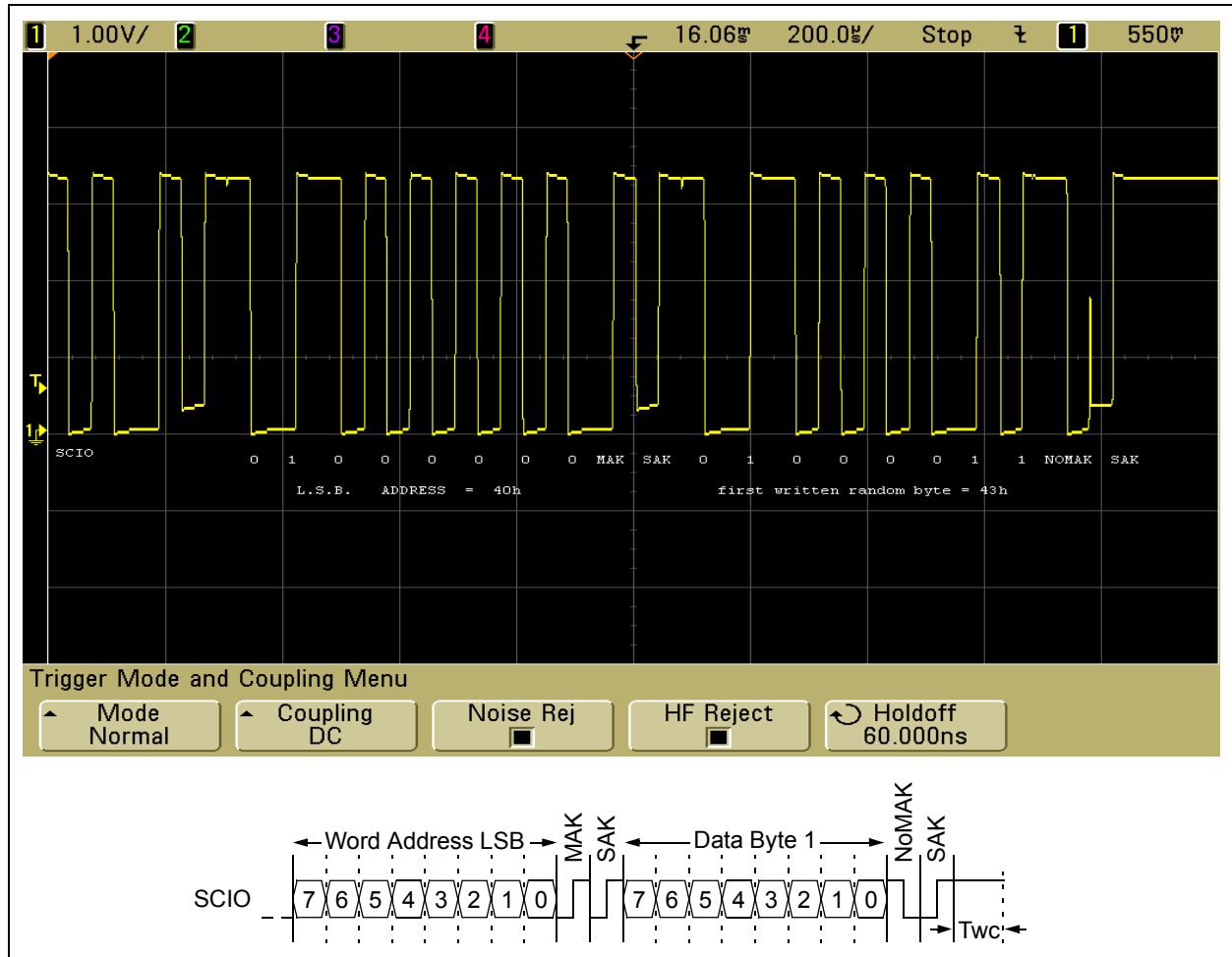
FIGURE 6: DATA BYTE AND STOP BIT
