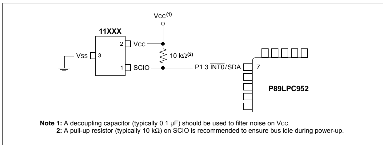
FIGURE 1: CIRCUIT FOR P89LPC952 MCU AND 11XXX SERIAL EEPROM
