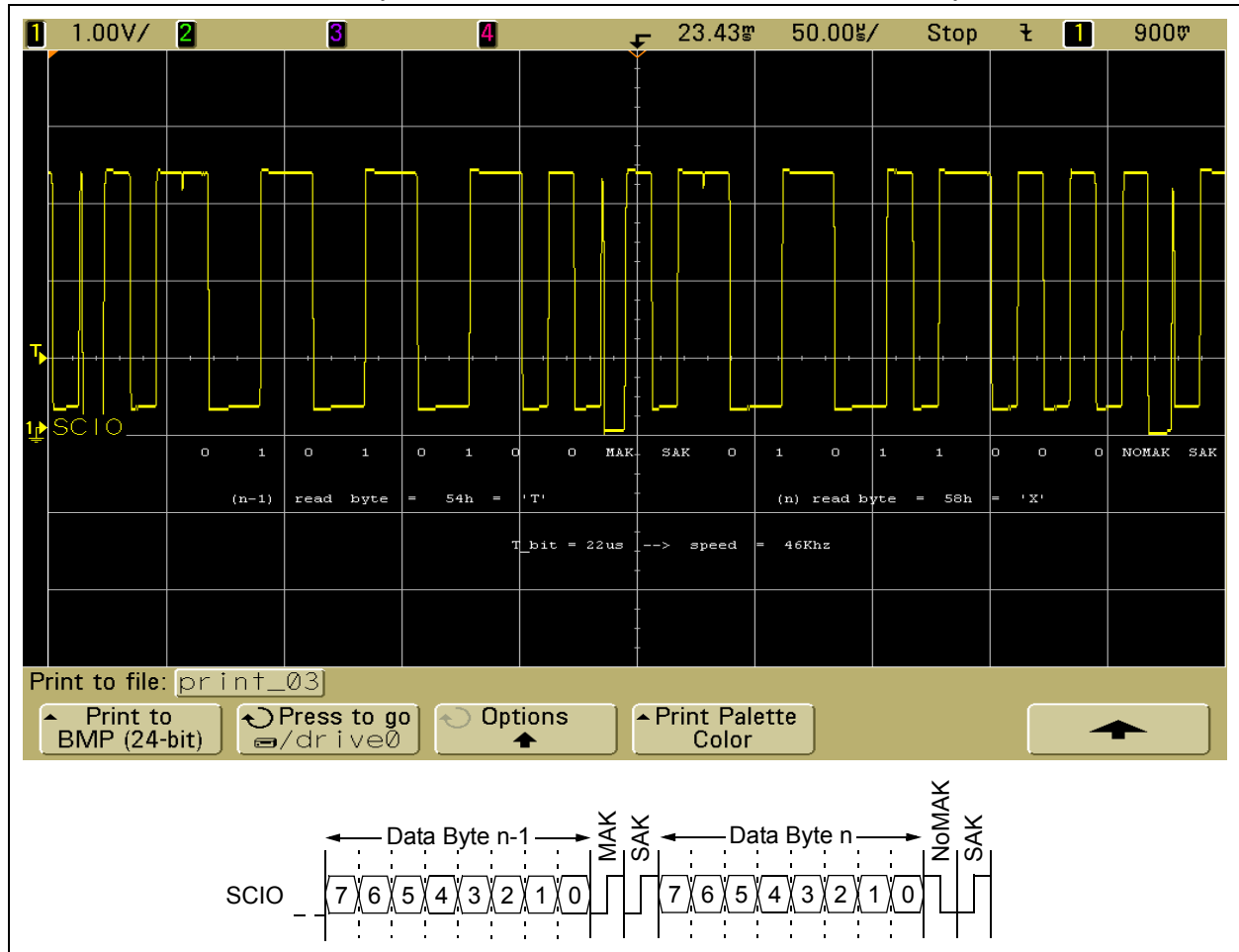
FIGURE 10: BYTE READ (DATA BYTES AND COMMAND TERMINATION)
